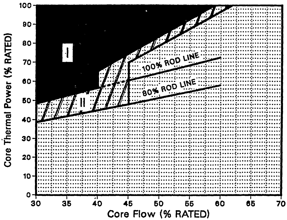
Figure 3.4.1.1.1-1 THERMAL POWER RESTRICTIONS
