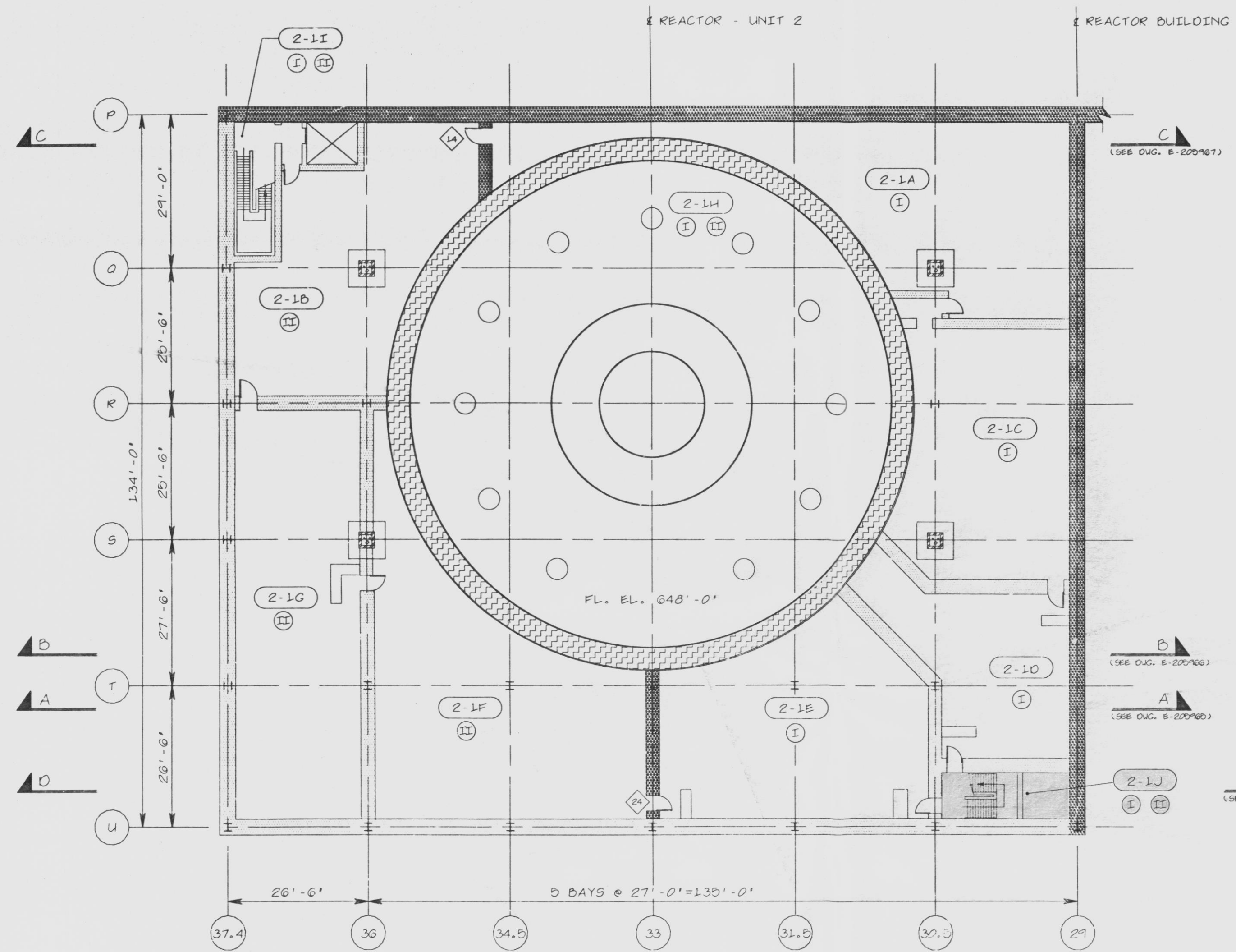
FLOOR PLAN @ EL. 645'-0"
