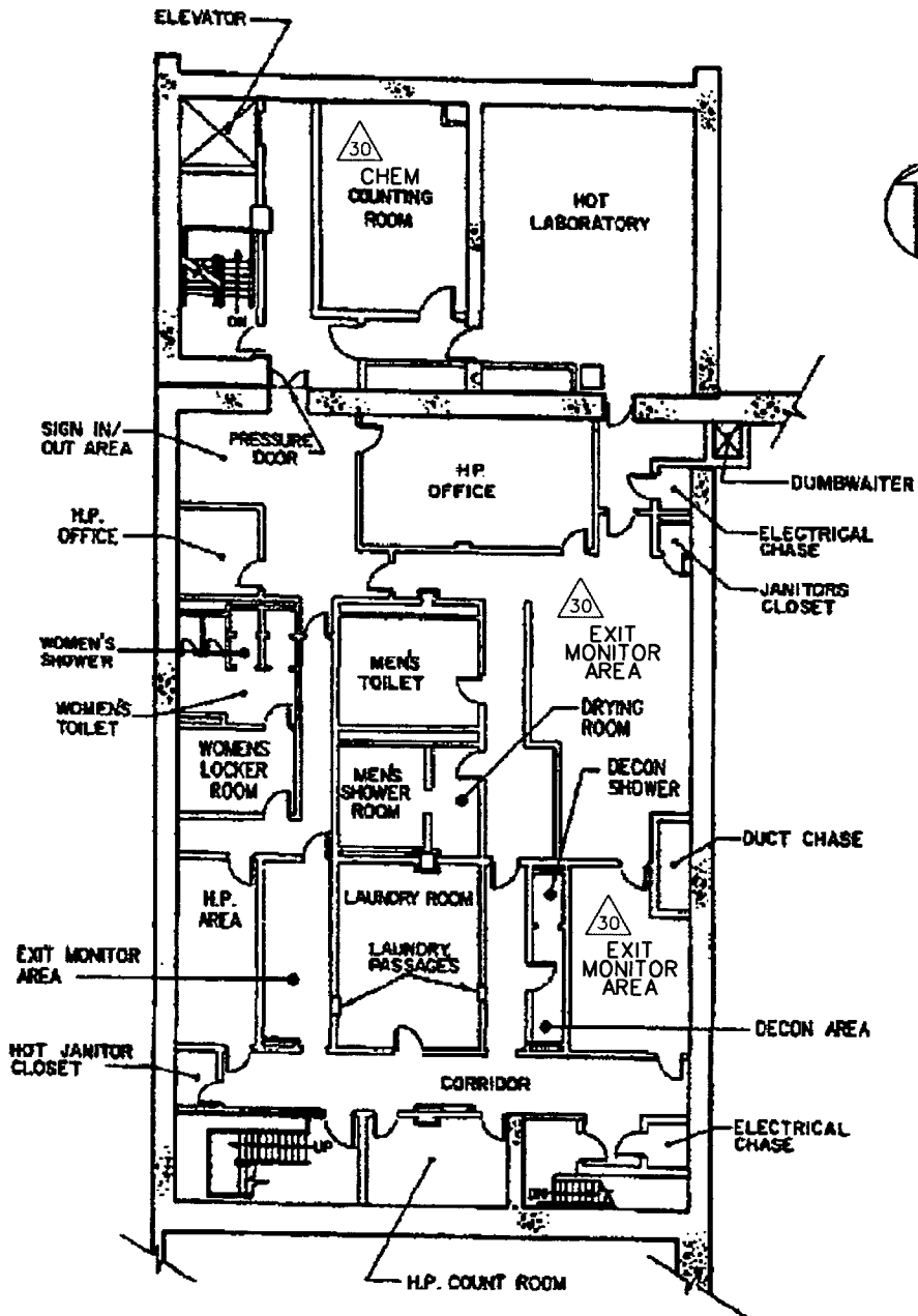
CONTROL BUILDING AT ELEVATION 1984
