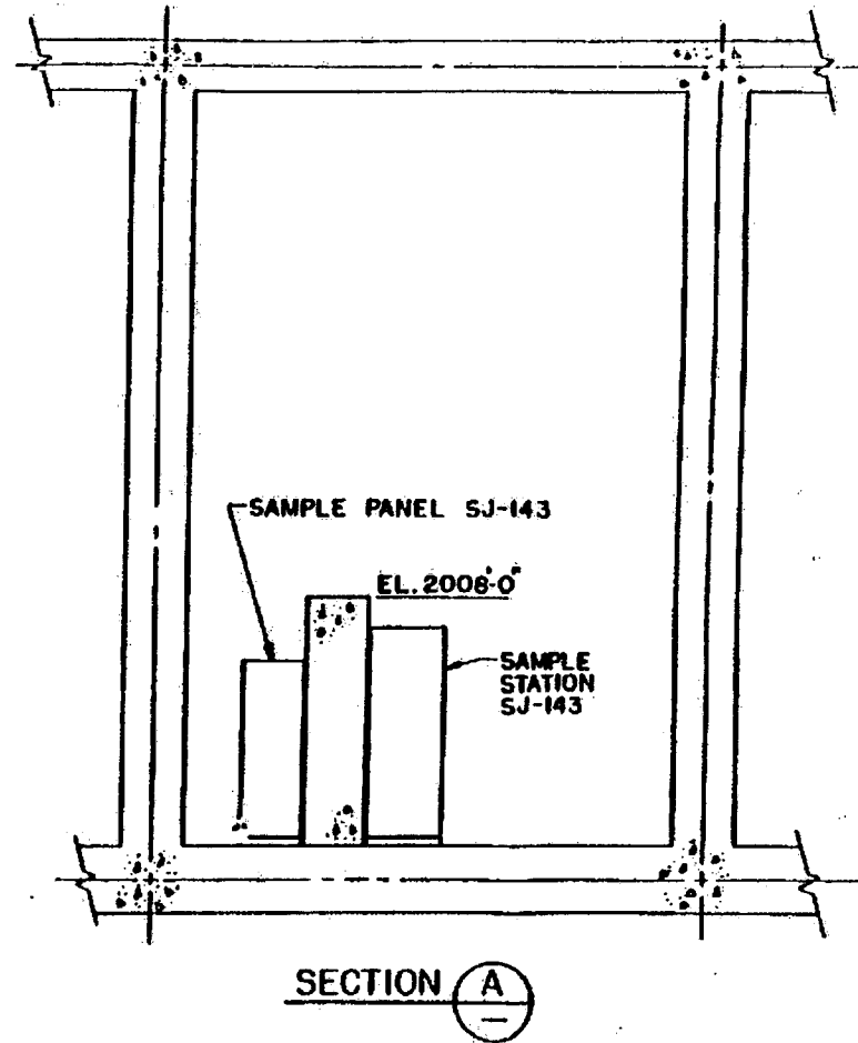
WOLF CREEK UPDATED SAFETY ANALYSIS REPORT FIGURE 12.3-1 TYPICAL VALVE COMPARTMENT ARRANGEMENT (SHEET 5)
