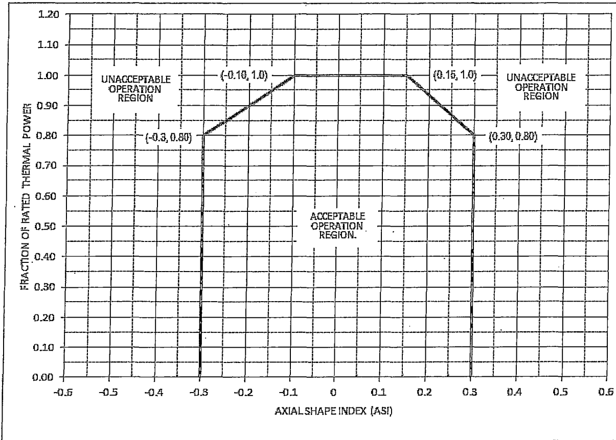
Figure 2.7-1 AXIAL SHAPE INDEX Operating Limits With Four Reactor Coolant Pumps Operating
