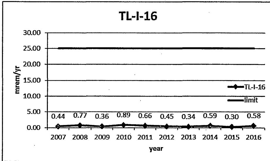
Figure 4.9 Annual Dose Trend at TL-I-16
