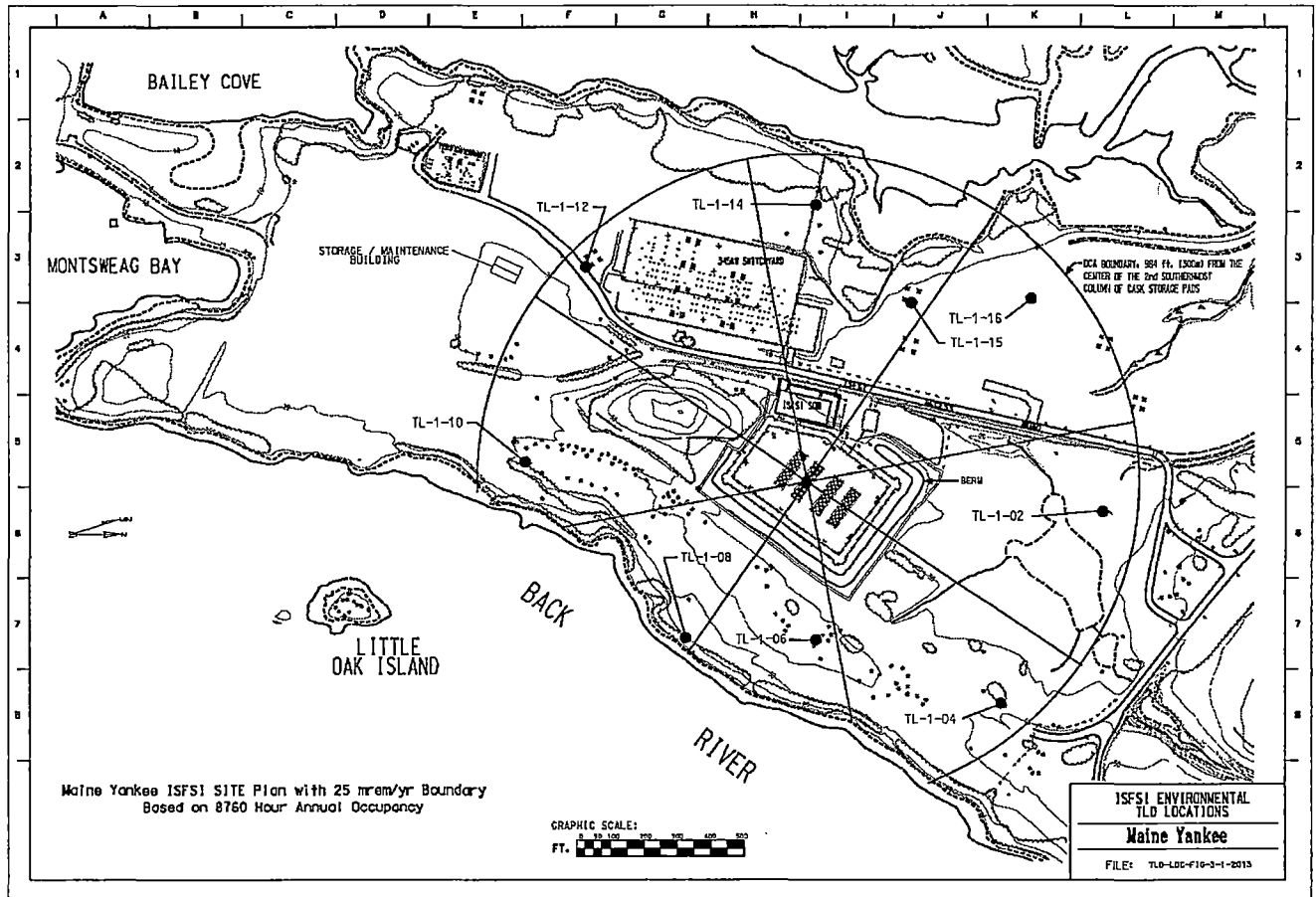
Figure 3.1 Radiological Environmental Monitoring Locations (within 0.28 km)
