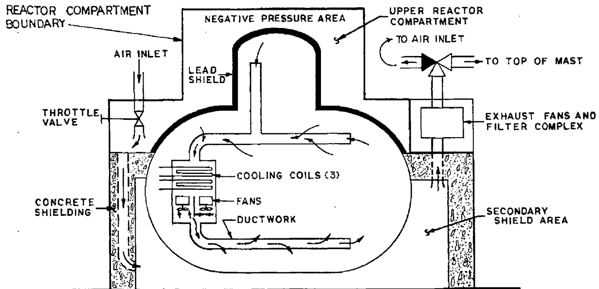
Figure 4-3 Reactor Compartment
