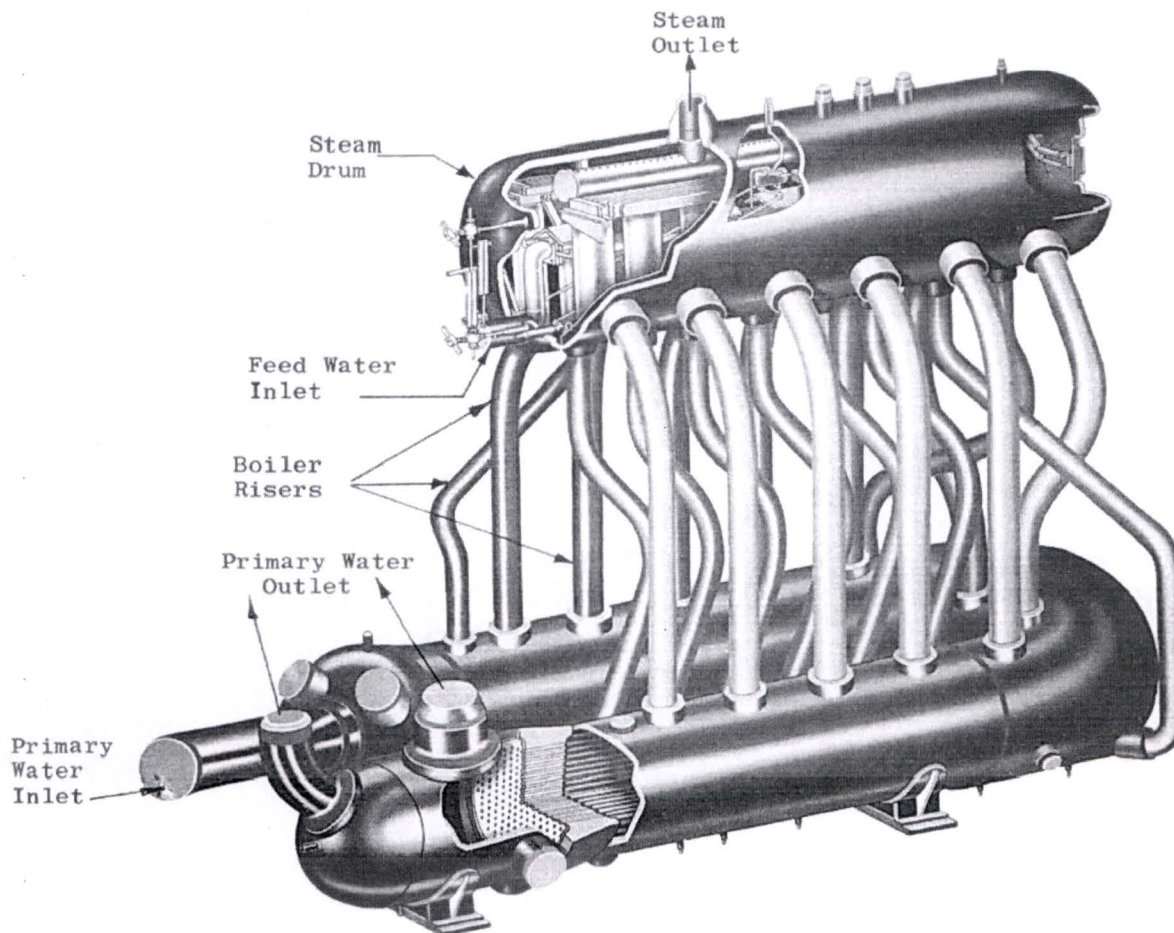
Figure 7-4 Steam Generator
