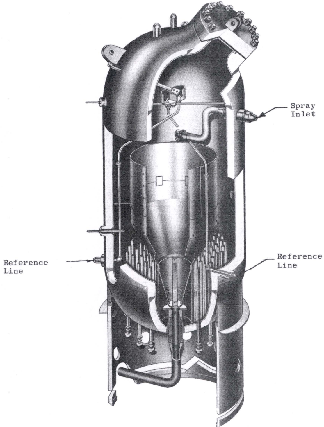
Figure 7-5 Pressurizer
