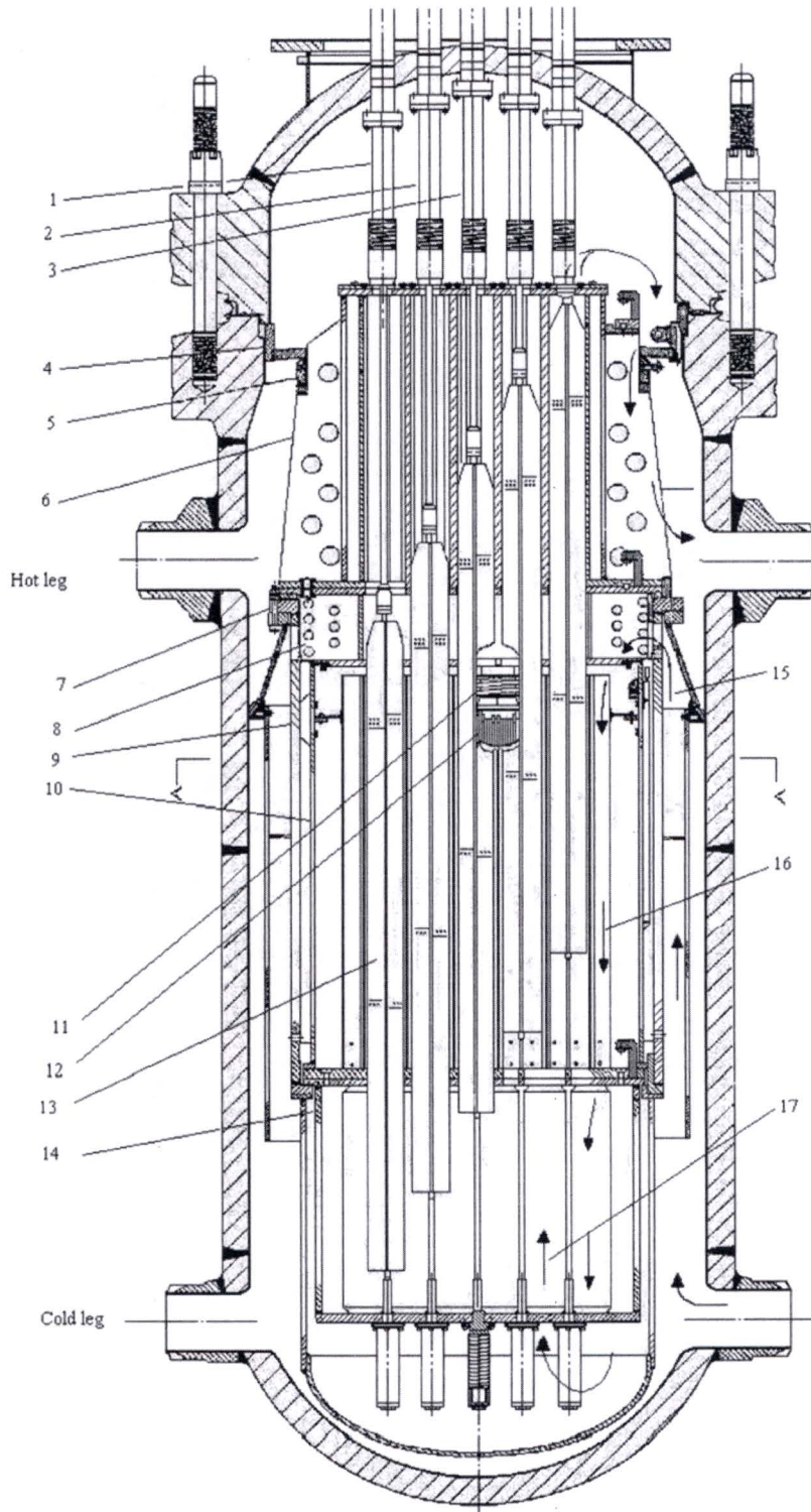
Figure 6-1 Reactor Internals
