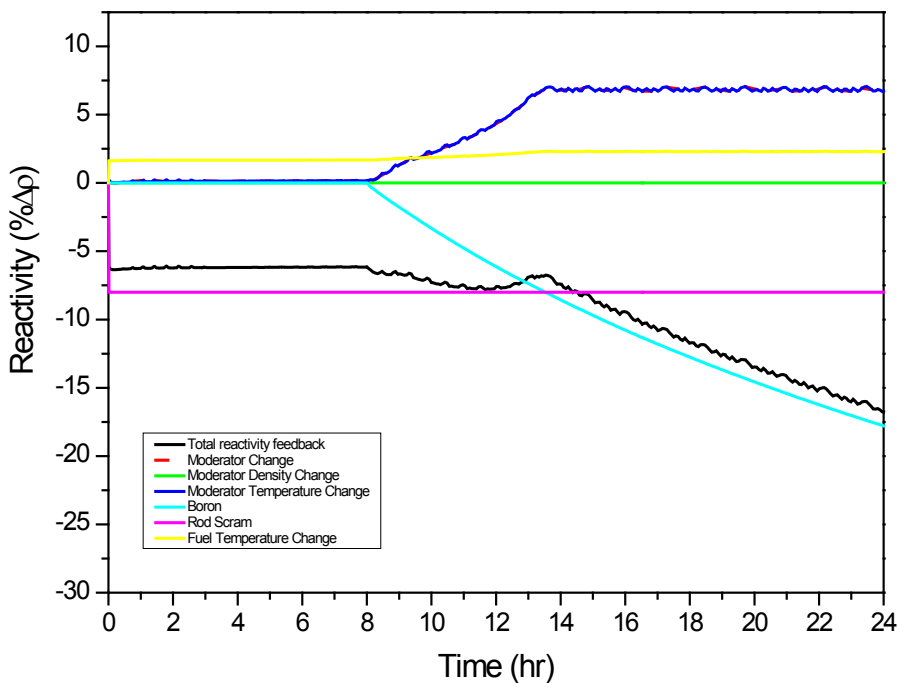
Figure A-22 Reactivity Changes during RCS Cooldown (No RCP Leak)
