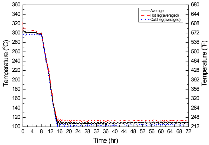
Figure A-12 RCS Temperature (Contingency Plan)
