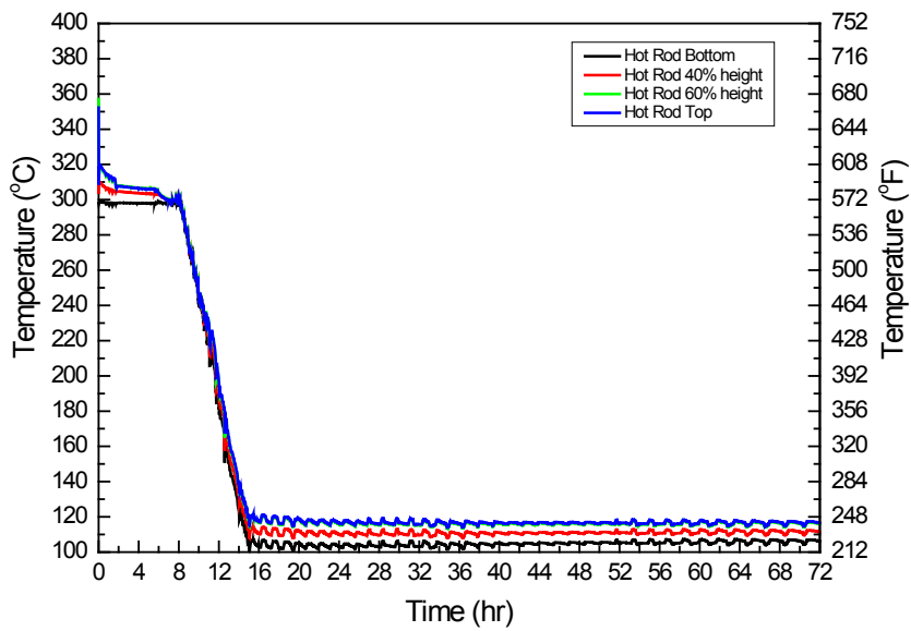
Figure A-18 Cladding Temperature (Contingency Plan)
