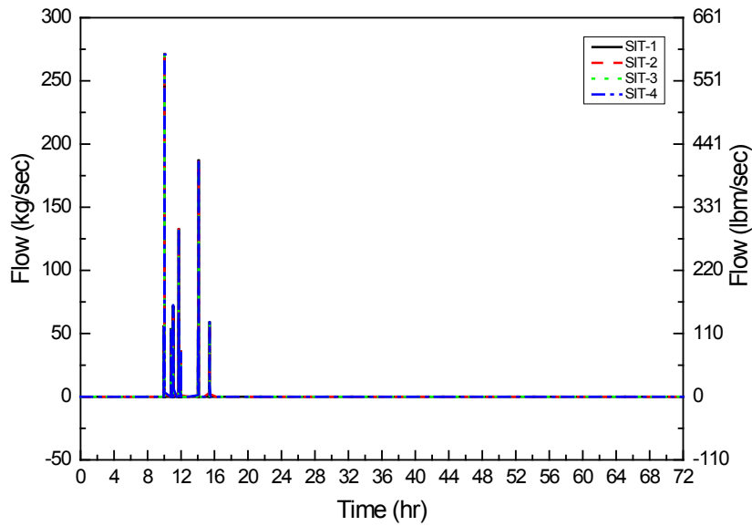
Figure A-13 SIT Flow (Contingency Plan)
