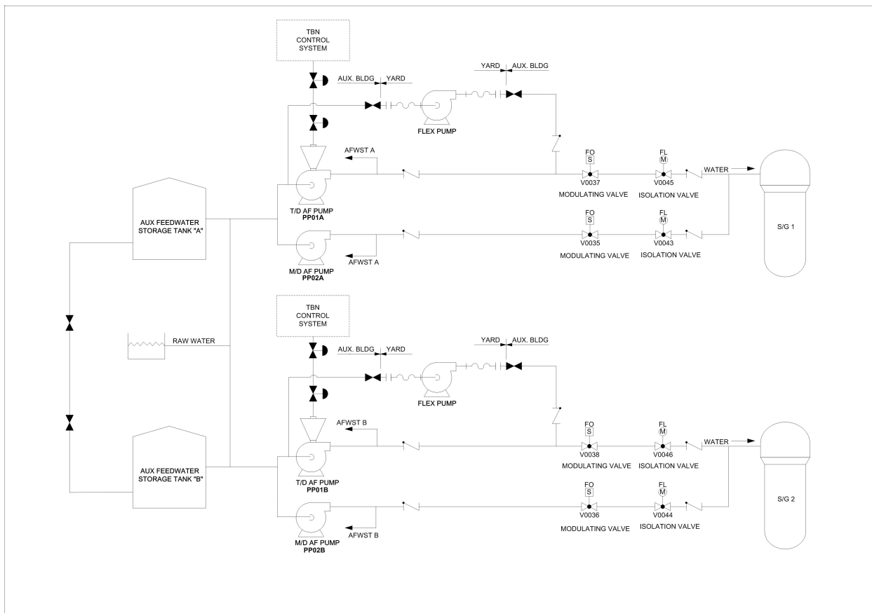
Figure 6-5 Water Supply System to the Secondary Side of SG
