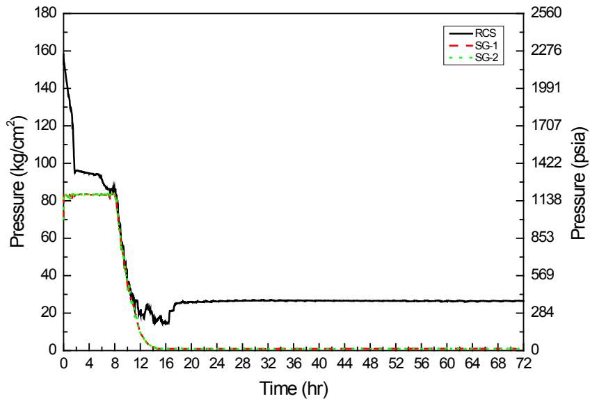
Figure A-11 RCS and Steam Generator Pressure (Contingency Plan)
