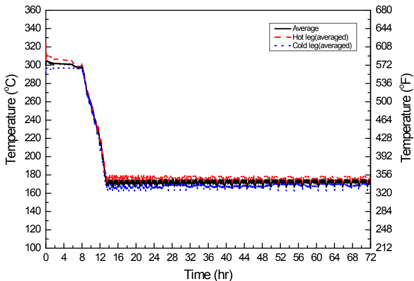
Figure A-2 RCS Temperature (Basic Strategy)
