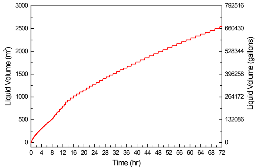
Figure A-10 Integration of AFW Flow (Basic Strategy)
