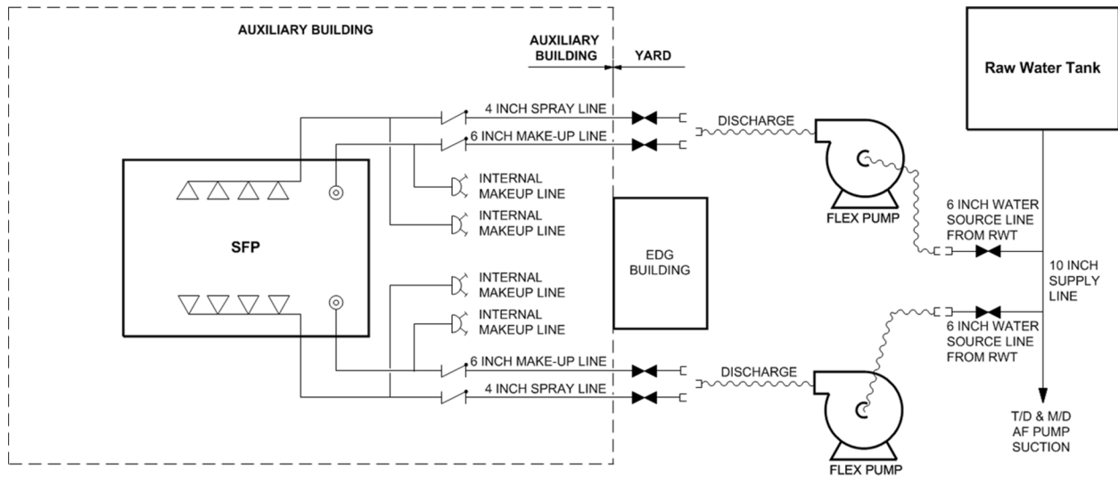
Figure 6-2 FLEX Pump Suction Source for SFP Makeup and Spray Line
