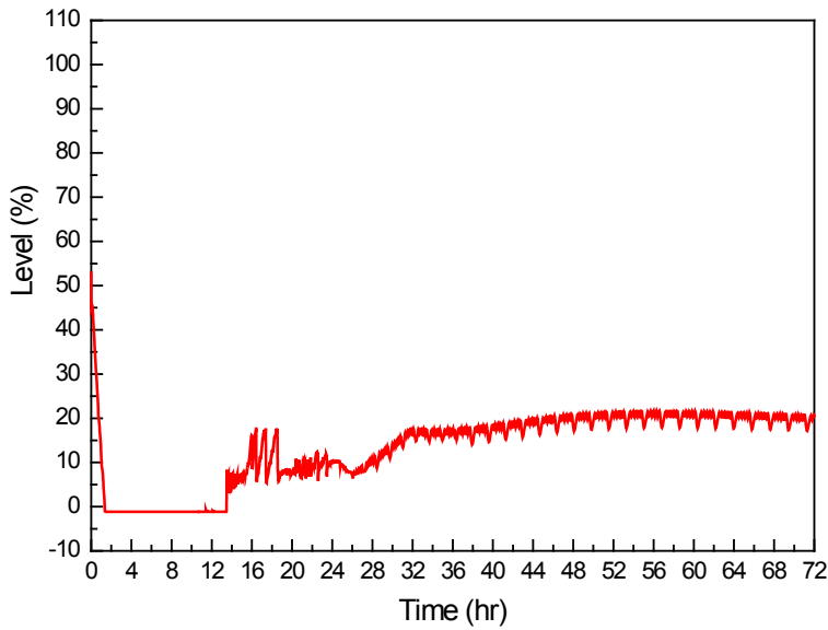
Figure A-6 RCS Pressurizer Water Level (Basic Strategy)
