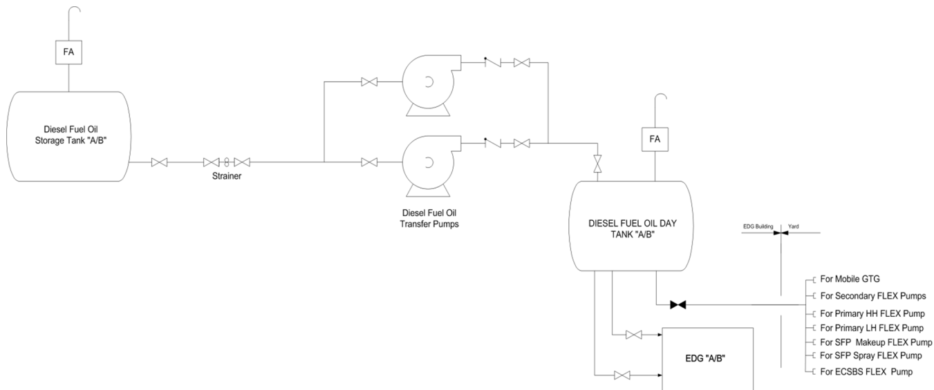
Figure 6-6 Fuel Oil Supply System to FLEX Pumps
