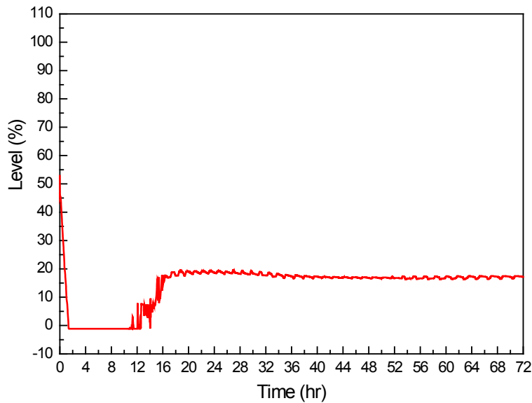
Figure A-16 Pressurizer Water Level (Contingency Plan)
