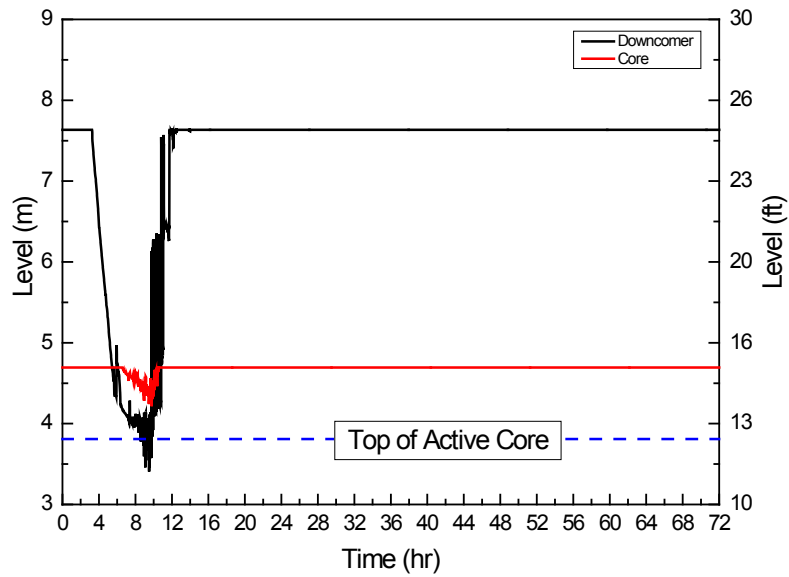
Figure A-17 Collapsed Downcomer and Core level (Contingency Plan)
