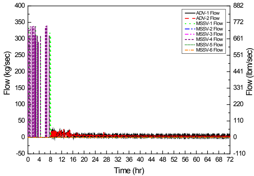
Figure A-19 MSADV, MSSV Flow (Contingency Plan)
