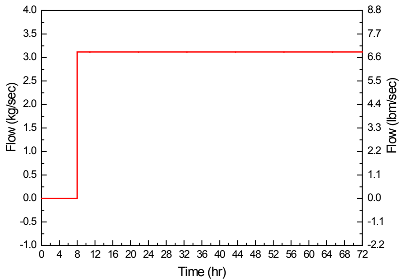
Figure A-14 Primary FLEX Pump Flow (Contingency Plan)
