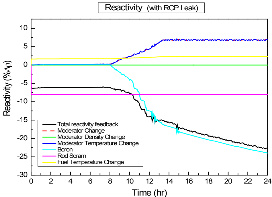
Figure A-21 Reactivity Changes during RCS Cooldown (with RCP Leak)
