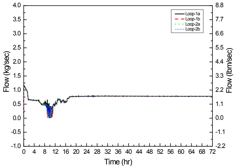
Figure A-15 RCS Leak Flow (Contingency Plan)
