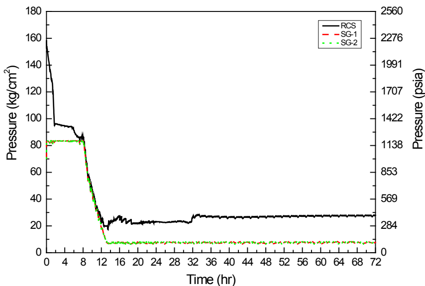
Figure A-1 RCS and Steam Generator Pressure (Basic Strategy)
