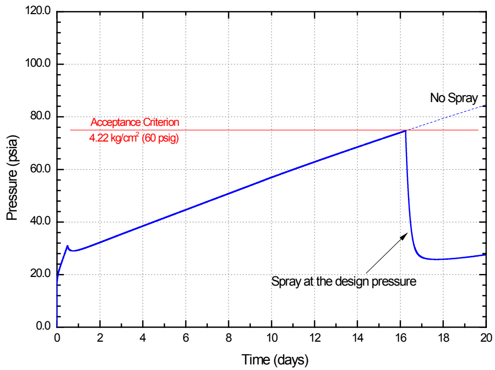
Figure 5-2 Containment Pressure for Full Power (RCP Seal LOCA)
