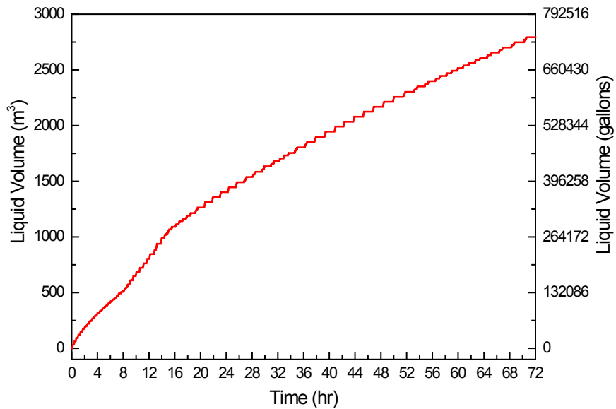
Figure A-20 Integration of AFW Flow (Contingency Plan)
