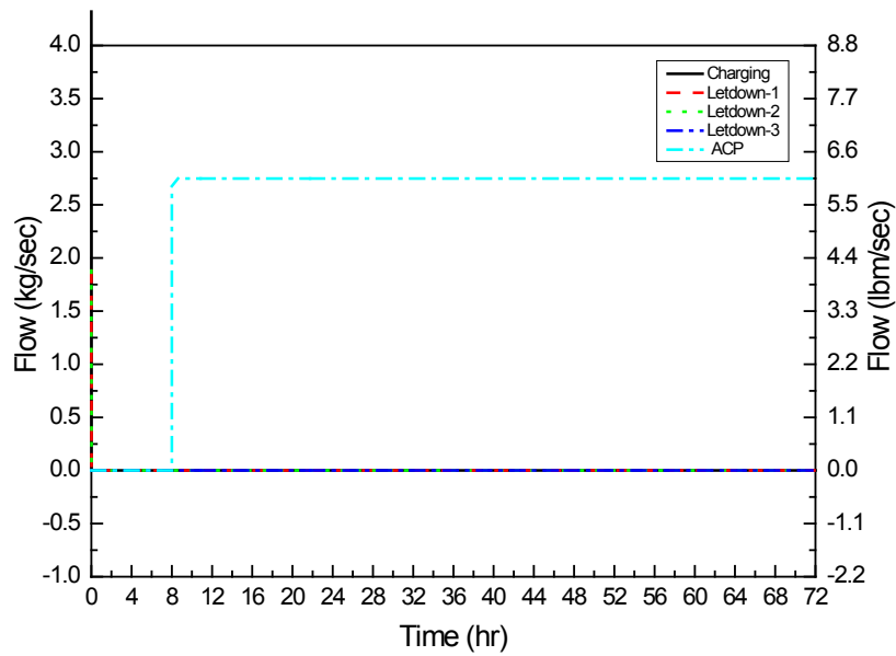
Figure A-4 ACP Flow (Basic Strategy)
