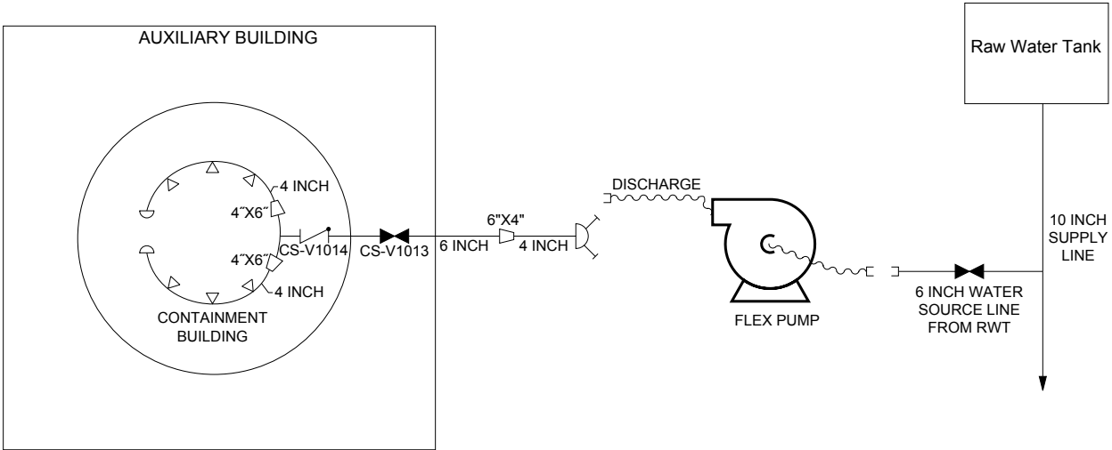
Figure 6-7 Flow Path for FLEX Connection to Deliver Water to Containment for ECSBS
