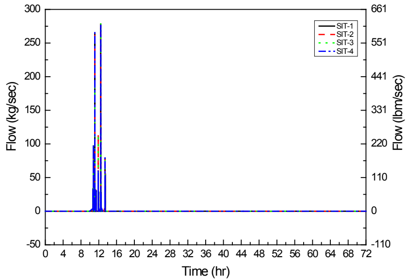
Figure A-3 SIT Flow (Basic Strategy)
