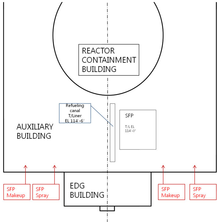
Figure 6-4 Layout of SFP Makeup and SFP Spray Line Connections
