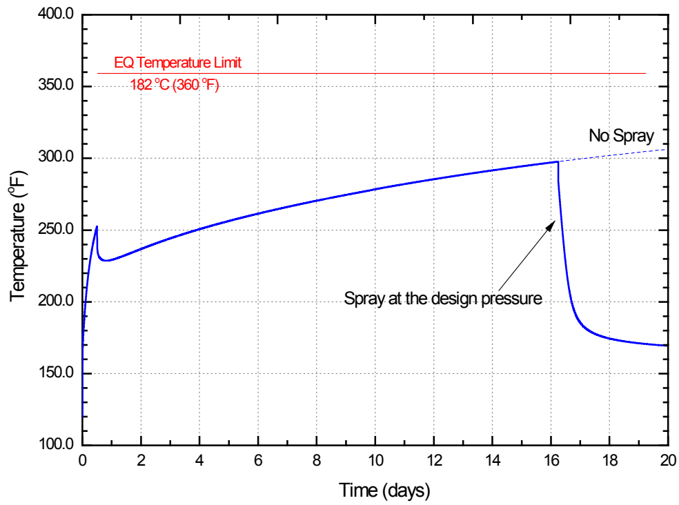
Figure 5-3 Containment Temperature for Full Power (RCP Seal LOCA)
