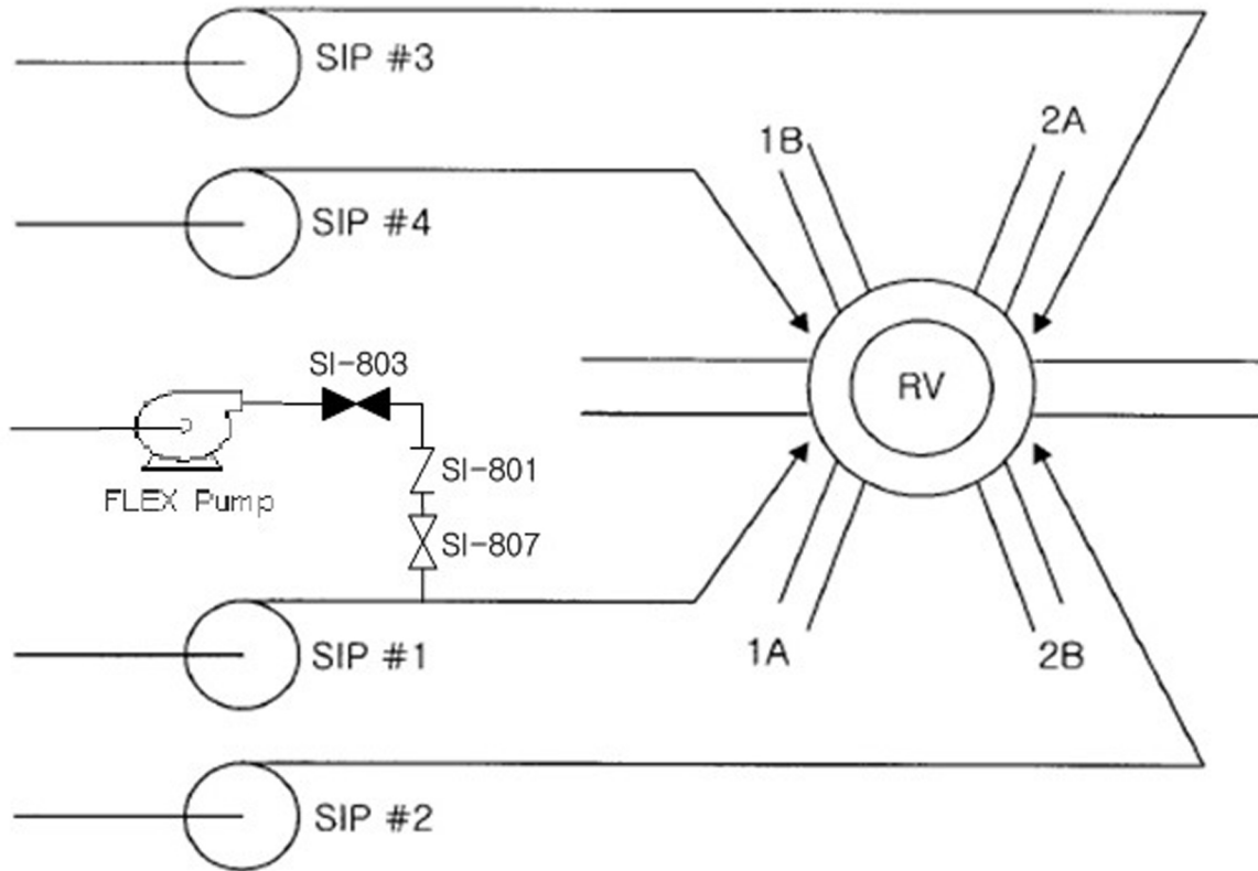
Figure 6-1 Primary Side FLEX Pump Connection into the Safety Injection System
