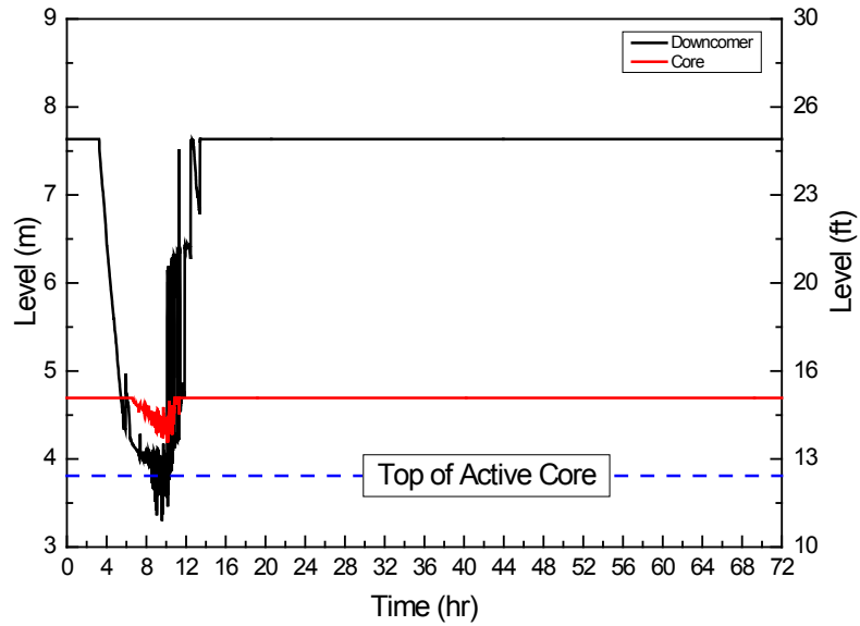
Figure A-7 Collapsed Downcomer and Core Level (Basic Strategy)
