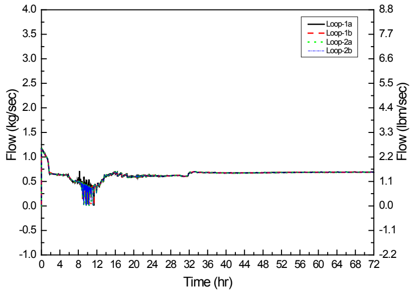
Figure A-5 RCS Leak Flow (Basic Strategy)
