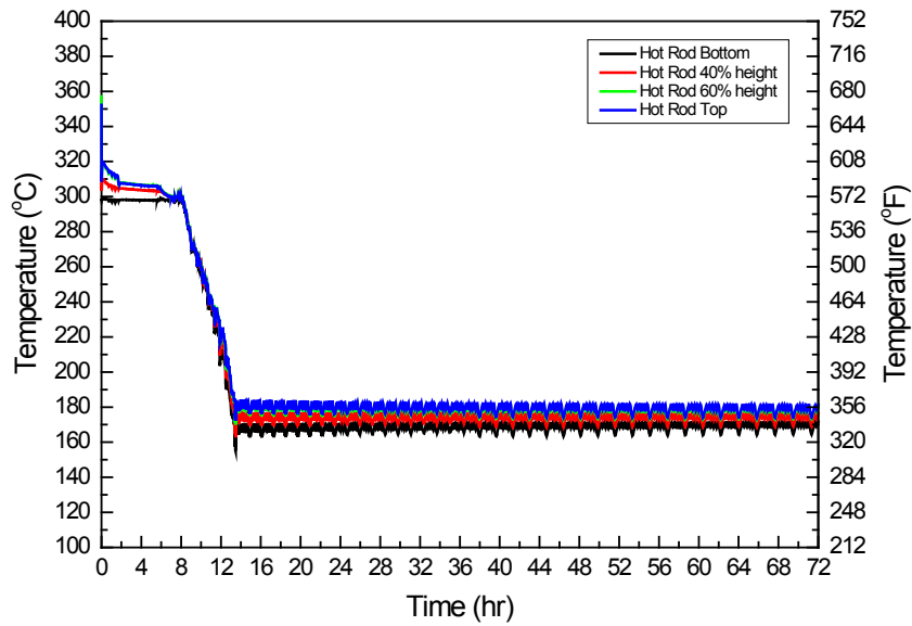
Figure A-8 Cladding Temperature (Basic Strategy)
