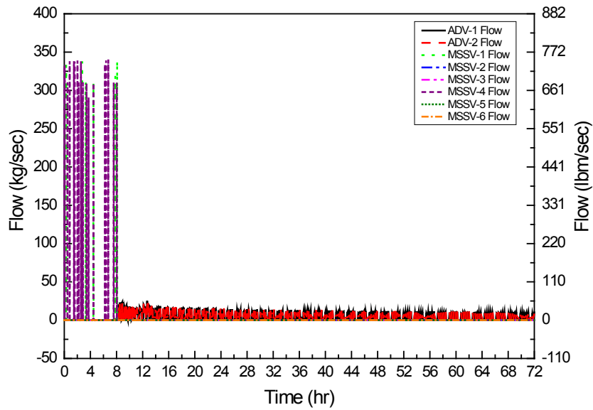
Figure A-9 MSADV, MSSV Flow (Basic Strategy)
