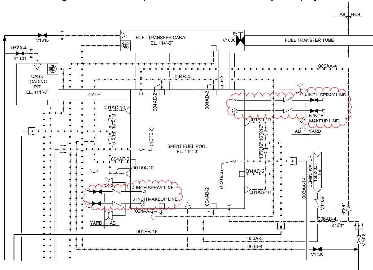
Figure 6-3 Connection for SFP Makeup and Spray Line
