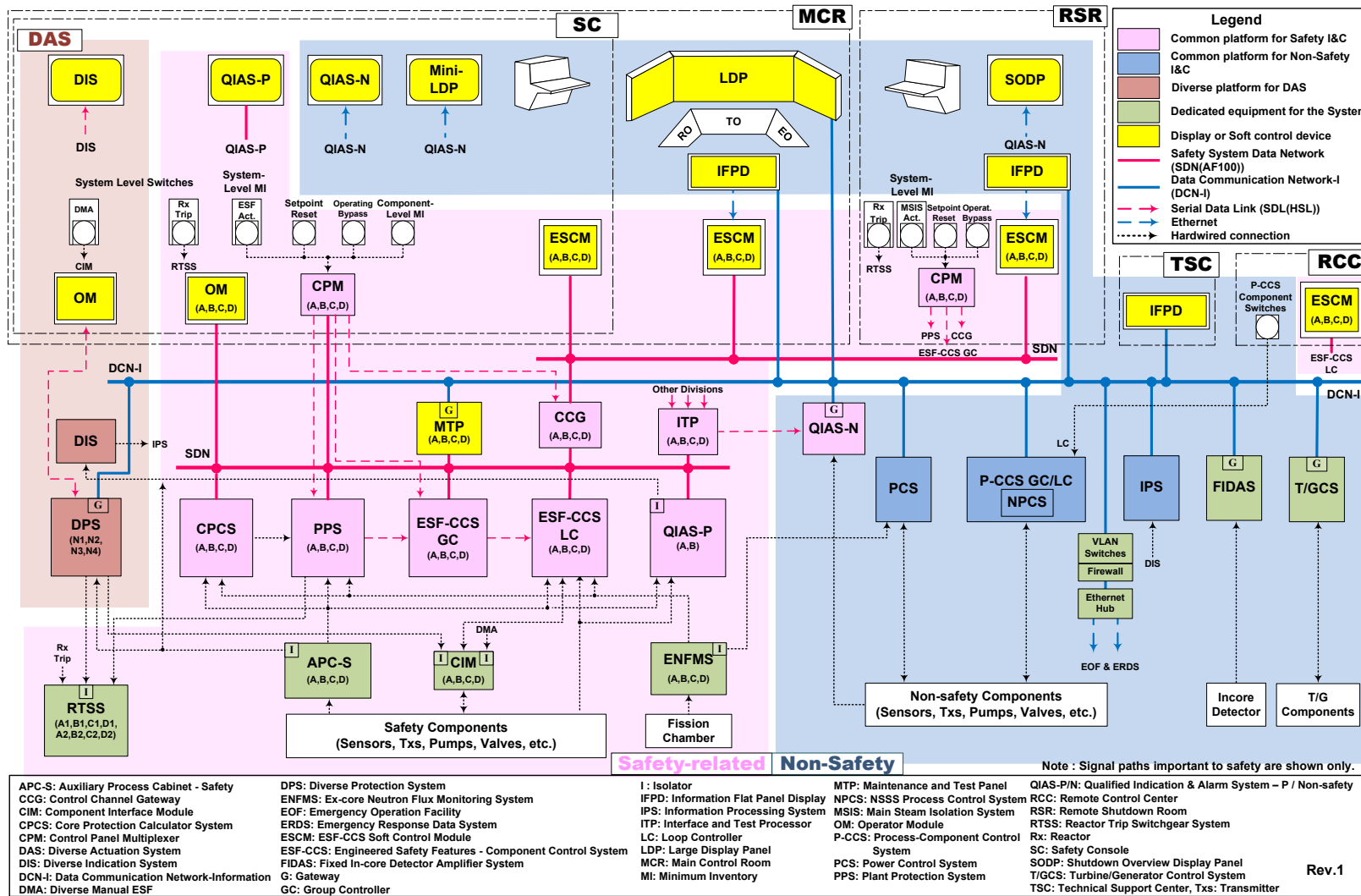
Figure 4-1 Overview of APR1400 I&C System Architecture
