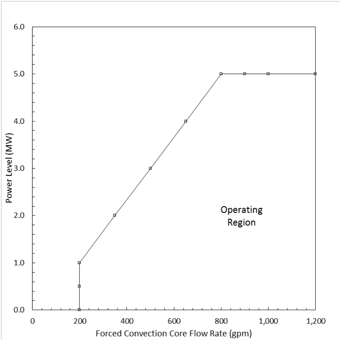
Figure 2-1 – Power–Flow Safety Limit Curve
