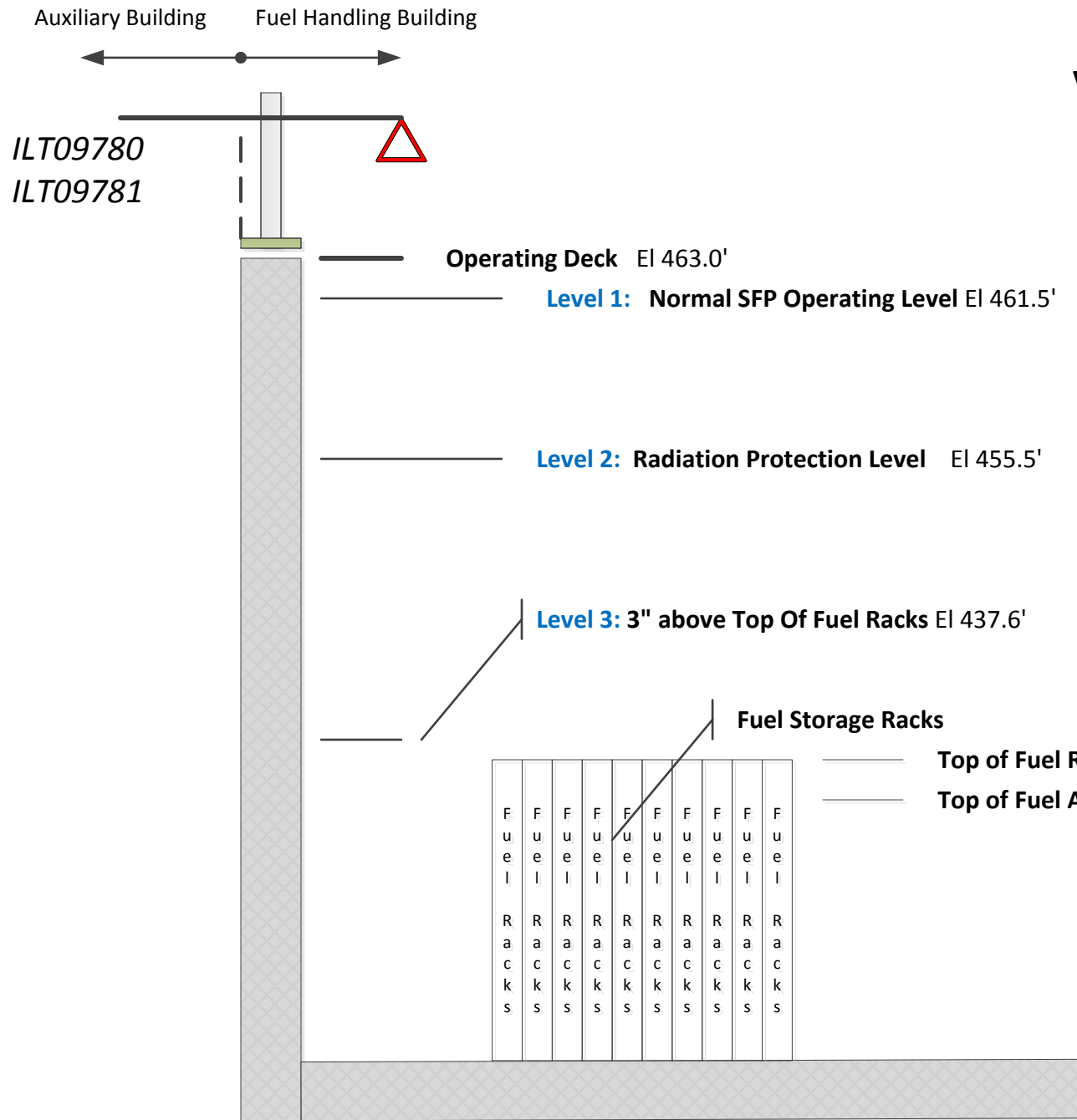
Spent Fuel Pool Elevation View
