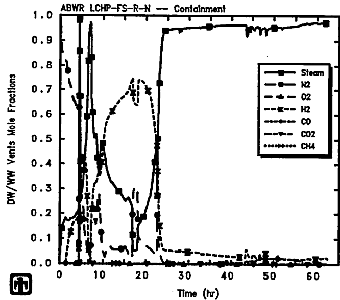
ABWR LCHP-FS-R-N: LC at HP, Firewater Spray, Passive Flood, Rupture ABRNXX 1/27/94 14:00:28 MELCOR HP
