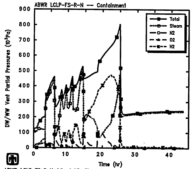
ABWR LCLP-FS-R-N: LC at LP, Firewater Spray, Passive Flood, Rupture ABWRNX 10/11/93 11:06:44 MELCOR HP
