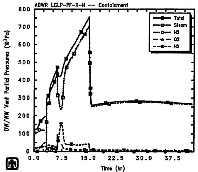
ABWR LCLP-PF-R-N: LC at LP, Passive Flood, Rupture ABWRNX 10/08/93 16:12:01 MELCOR HP
