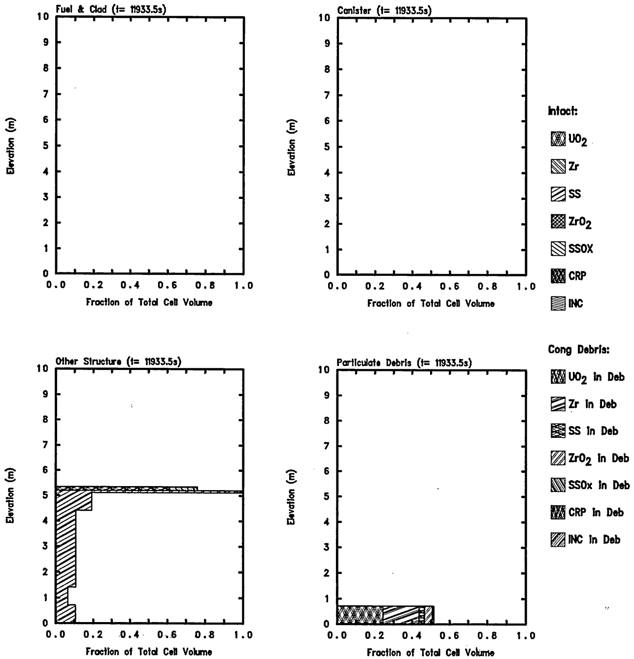
Figure 5.1.8. Core Ring 1 Fuel/Clad (upper left), Canister (upper right), Other Structure (lower left) and Particulate Debris (lower right) Component Material Masses Predicted by MELCOR for LCLP-PF-R-N Sequence
