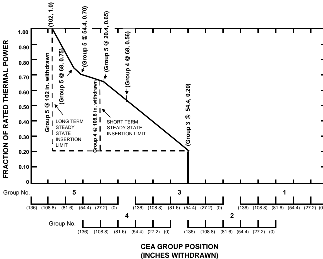
FIGURE 3.1-2 CEA Group Insertion Limits vs. THERMAL POWER
