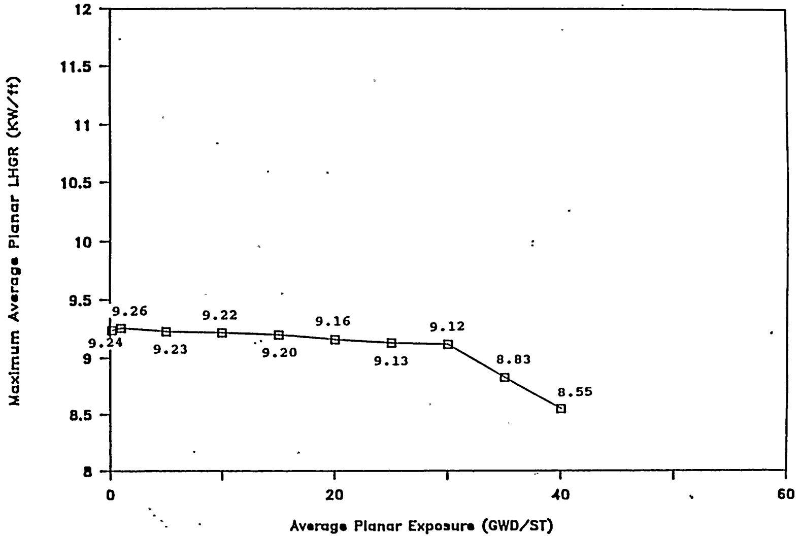
Figure A NMP-1 MAPLHGR Limits (GE 8DNB277)
