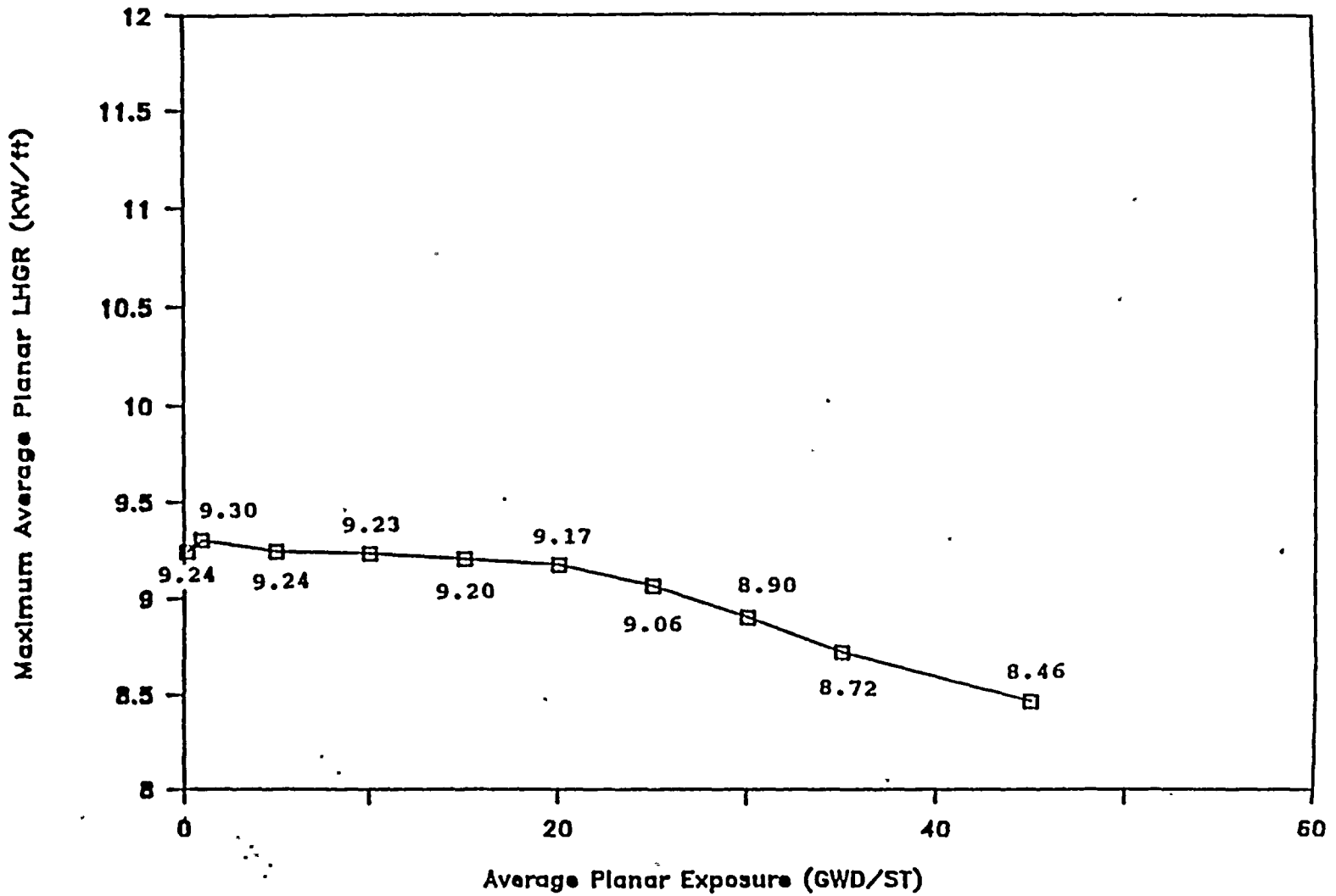
Figure B NMP-1 MAPLHGR Limits (GE P8DNB277)
