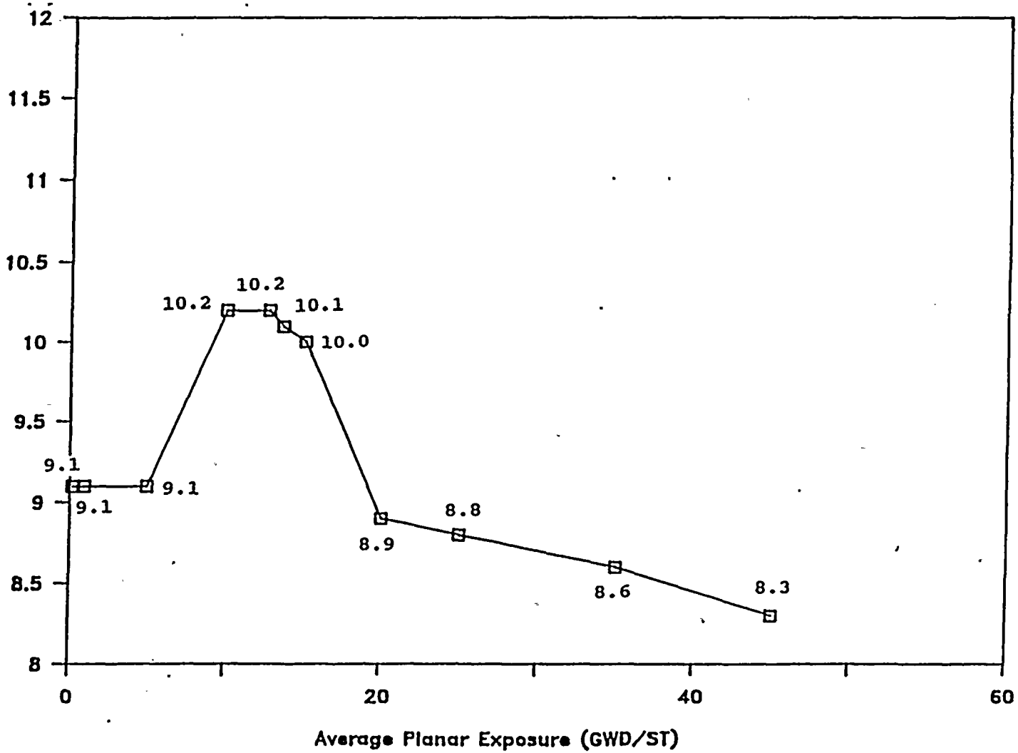
Figure C NMP-1 MAPLHGR Limits (GE7 P8DRB299)
