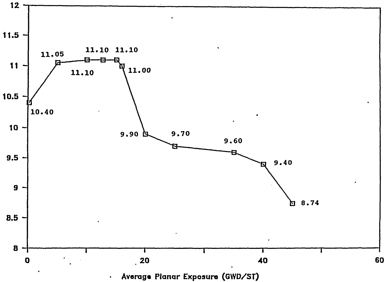
Figure D NMP-1 MAPLHGR Limits (GE8 BD321B)
