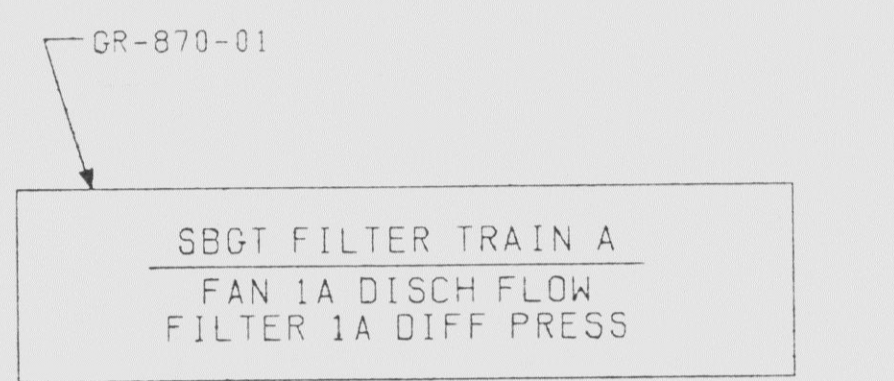
DETAIL "B" NAMEPLATE TO BE 4.00" X 1.00" GRAVPLCY. WHITE WITH BLACK CORE PER HERMES CO. NO. 200-12. 1/8" HIGH CHARACTERS TO BE ENGRAVED AS SHOWN.
