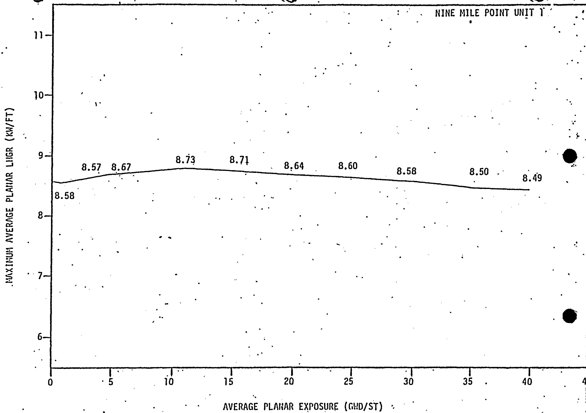
Figure 3.1.7a MAXIMUM ALLOWABLE AVERAGE PLANAR LHGR APPLICABLE TO 8DB250 FUEL AS DESCRIBED IN REFERENCE 8. Amendment No. 31, 41, 47
