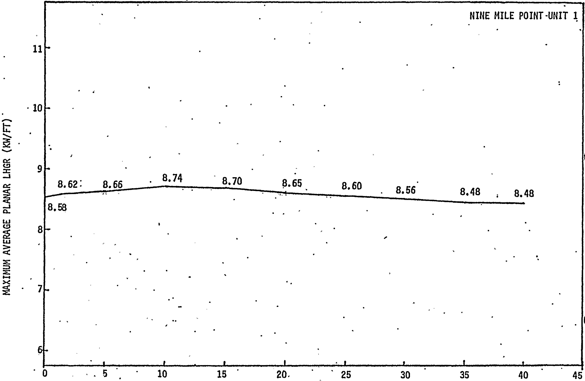
Figure 3.1.7b Maximum Allowable Average Planar LHGR Applicable to 8DB274L and 8DB274H Fuel as described in Reference 8.
