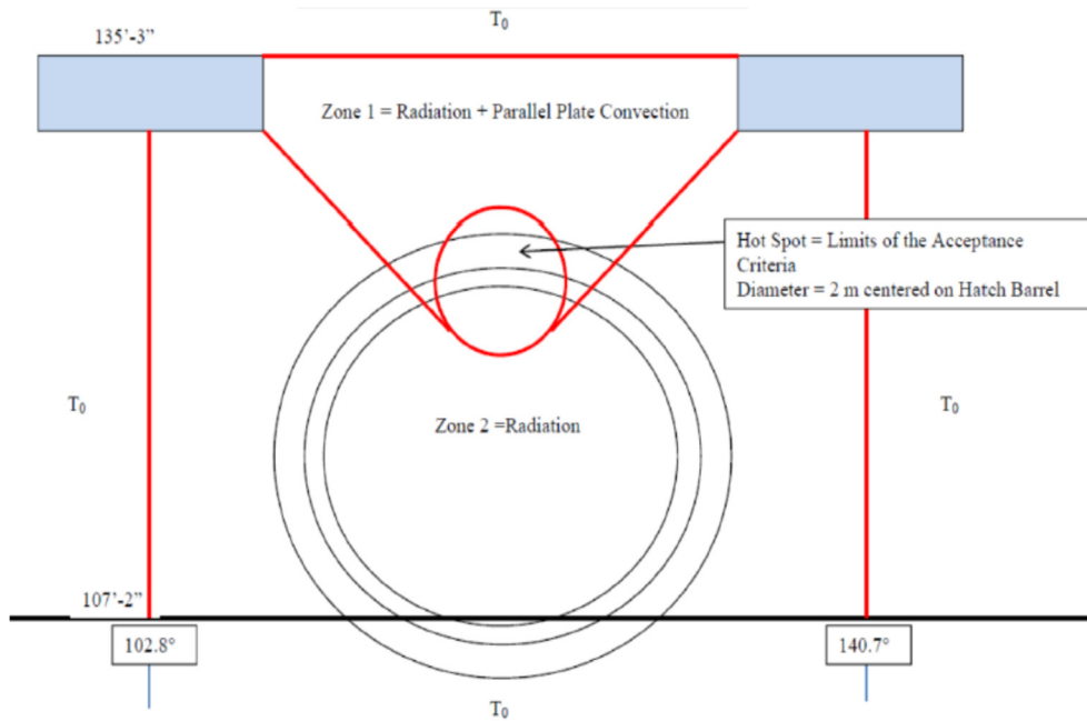
Figure 3-3. Temperature Distribution 2: Hot Spot on the Containment Shell at the Ceiling Vent Exit
