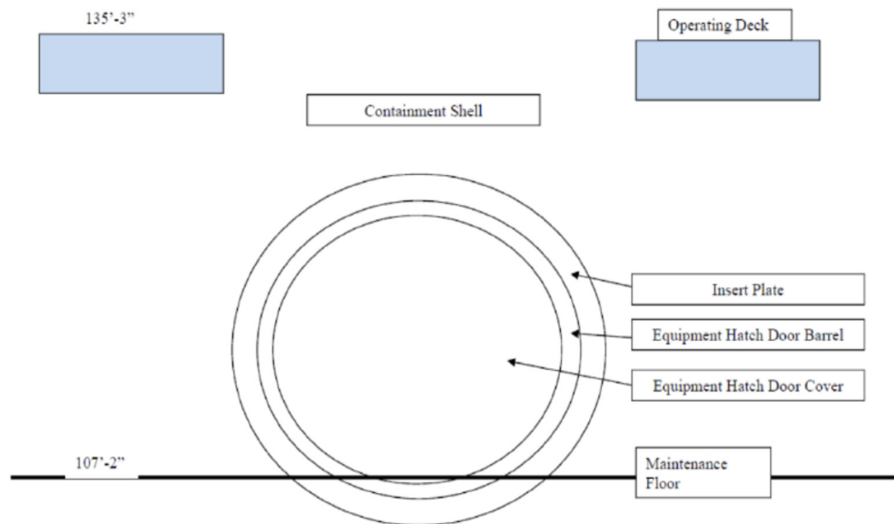
Figure 3-1. Component Layout for Temperature Distribution
