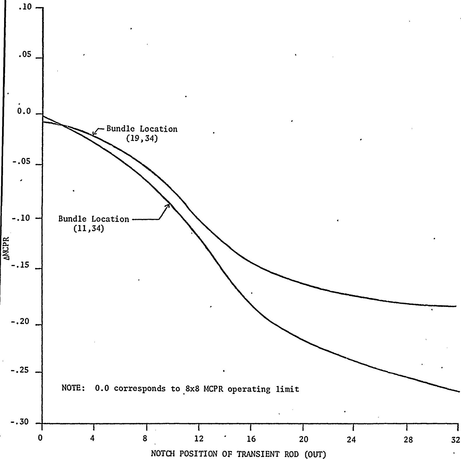
Figure 1. NMP-1 Cycle 3 Notch Position of Transient Rod versus \Delta\text{MCPR} for 7x7 Fuel
