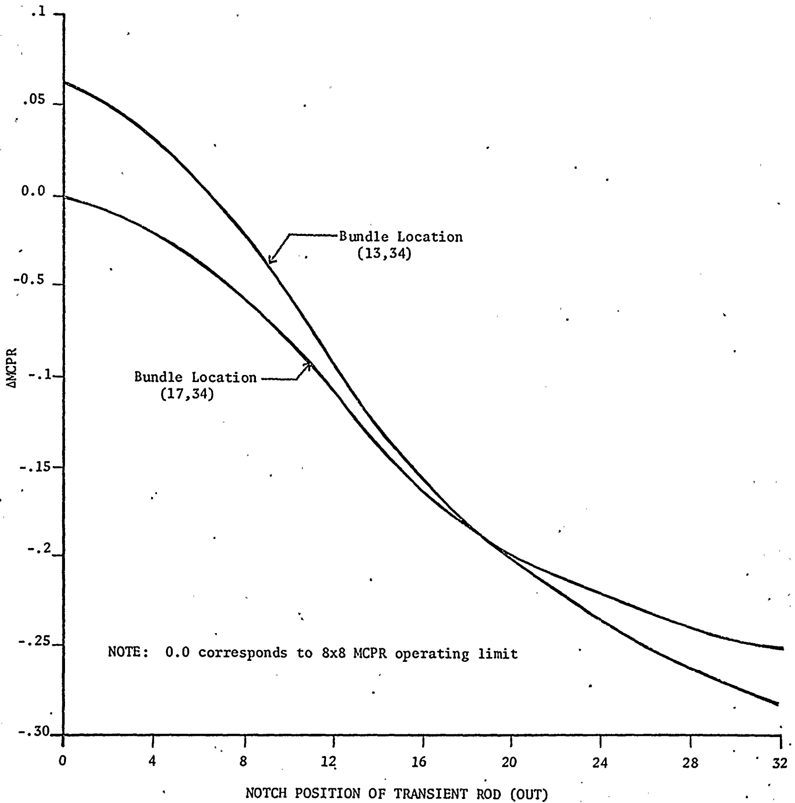
Figure 2. NMP-1 Cycle 3 Notch Position of Transient Rod versus ΔMCPR for 8x8 Fuel
