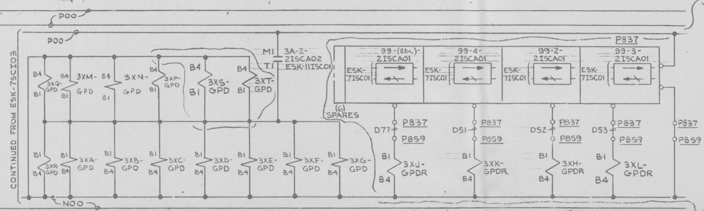
CONTAINMENT ISOL VALVE OFF NORMAL STATUS DISPLAY, CKT 25CIA02 (GREEN)
