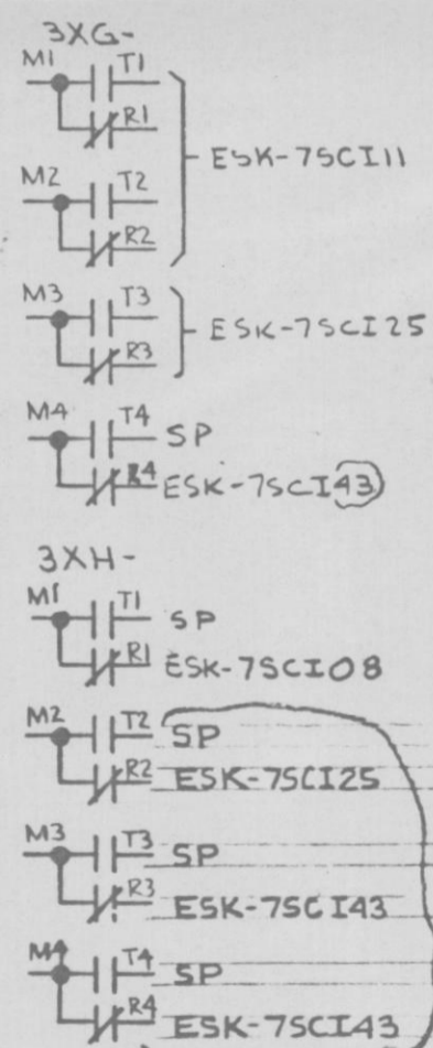
CONTAINMENT ISOL VALVE OFF NORMAL STATUS DISPLAY, CKT 25CIA02 (GREEN)
