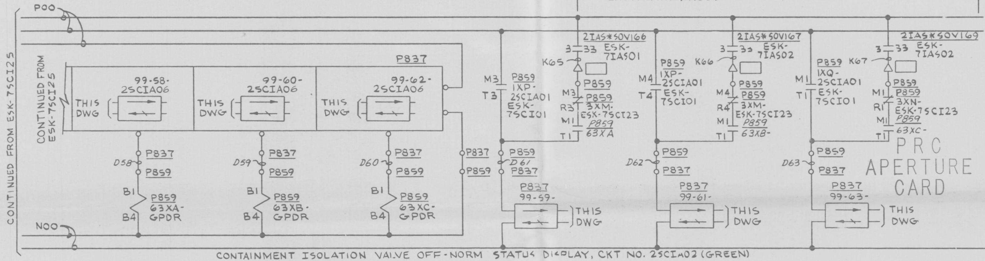
CONTAINMENT ISOLATION VALVE OFF-NORM STATUS DISPLAY, CKT NO. 25CIA02 (GREEN)
