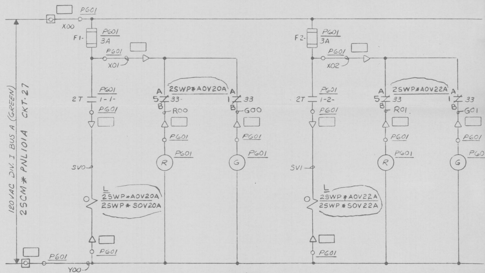
RHS PUMP PIA SEAL AND BRG COOLER 25WP*AOV20A/22A CKT - 25WPA32 (GREEN)
