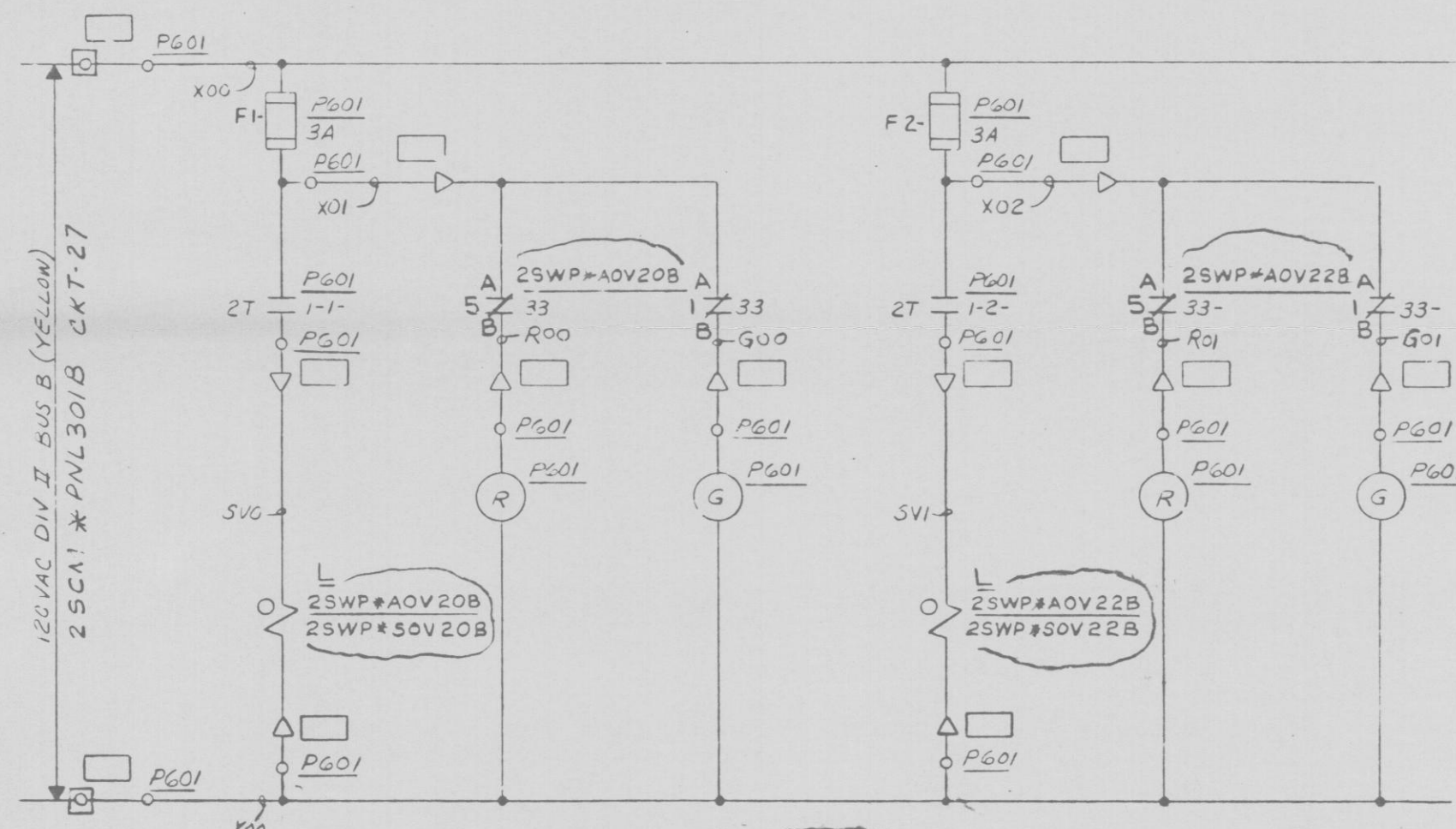
RHS PUMP PIB & PIC SEAL AND BRG COOLER 25WP*AOV20B/22B CKT - 25WPB32 (YELLOW)
