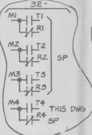
DIV II VALVES CKT-2CMSB03 (YELLOW)
