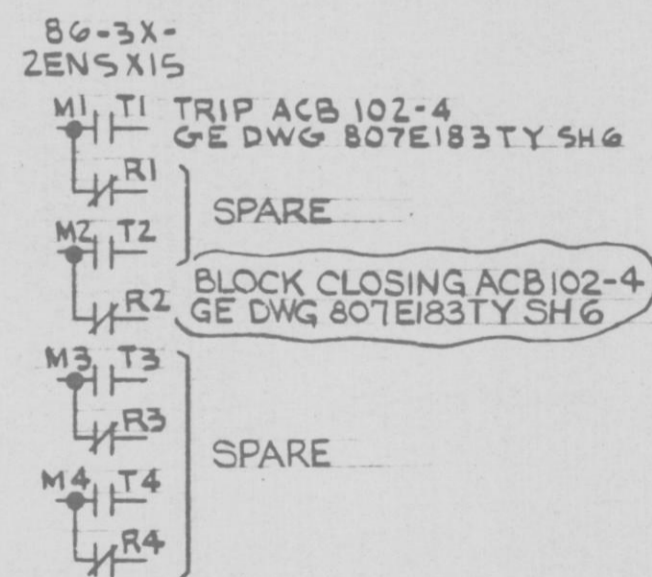
NORMAL SPLY BREAKER ACB 102-4, CKT NO. 2ENSXIS (PURPLE)
