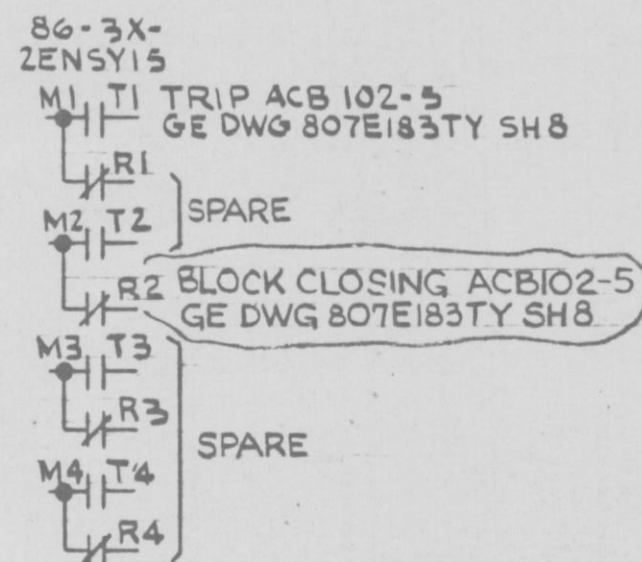
ALTERNATE SPLY BREAKER ACB 102-5, CKT NO. 2ENSYIS (PURPLE)
