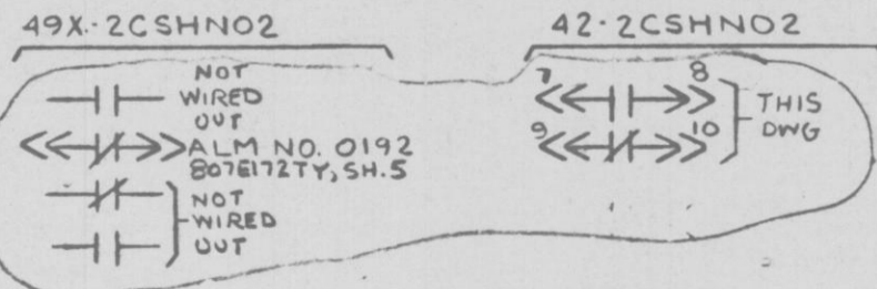
HPCS WATER LEG PMP 2CSH * P2 (GE. NO. E22-C003) CKT 2CSHNO2 MCC 2EHS * MCC 201 (PURPLE)
