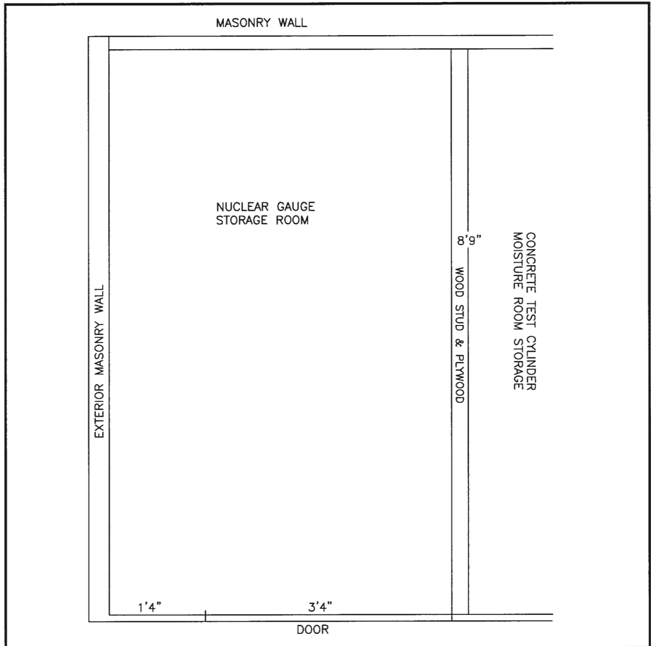
FIGURE 1.0 DETAILED SITE PLAN NUCLEAR GAUGE STORAGE ROOM TTL ASSOCIATES, INC. 44265 PLYMOUTH OAKS BLVD PLYMOUTH, MICHIGAN 48170
