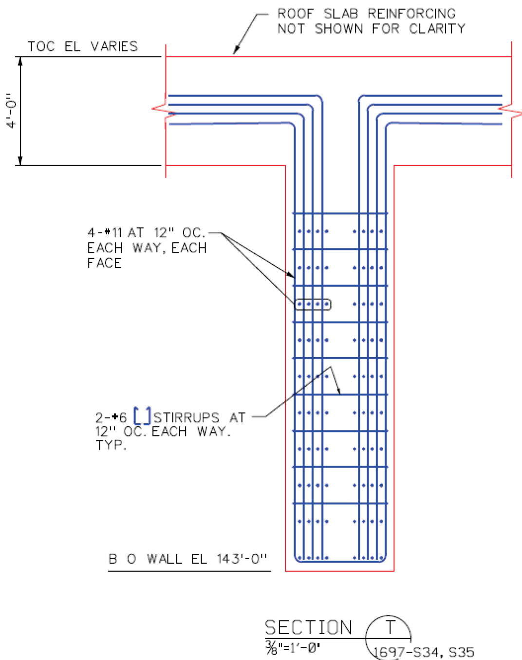
Figure 3B-13: RXB Reinforcement Section View of Stiffener Wall on Grid Line 3
