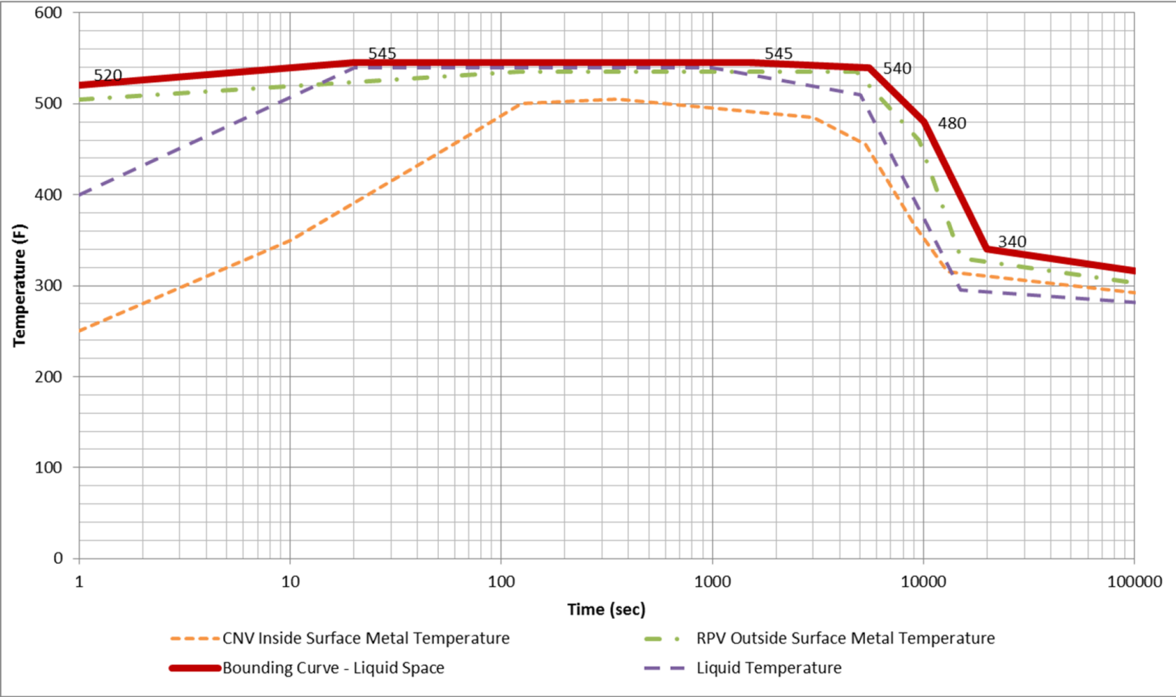
Figure 3C-1: Containment Liquid Space Metal and Liquid Temperatures with Bounding Curve (Zones A and B)
