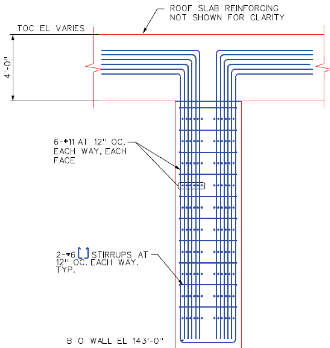
Figure 3B-17: RXB Reinforcement Section View of 4 ft Thick Wall on Grid Line 4
