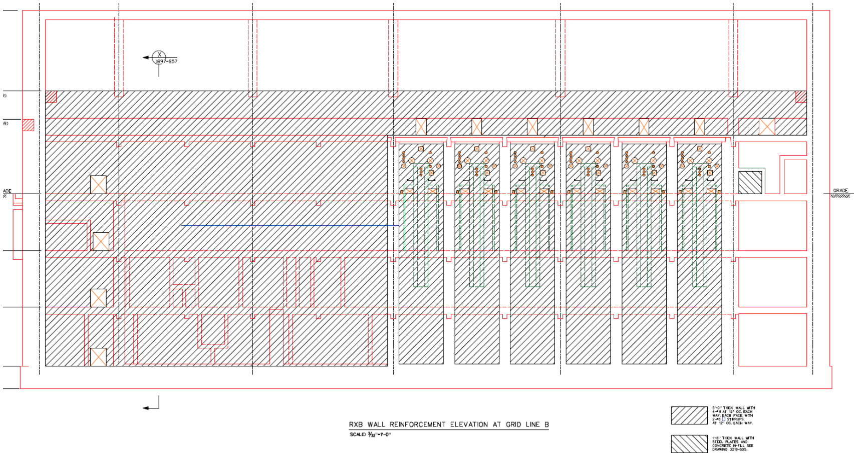
Figure 3B-46: RXB Reinforcement Elevation at RXB Wall at Grid Line B
