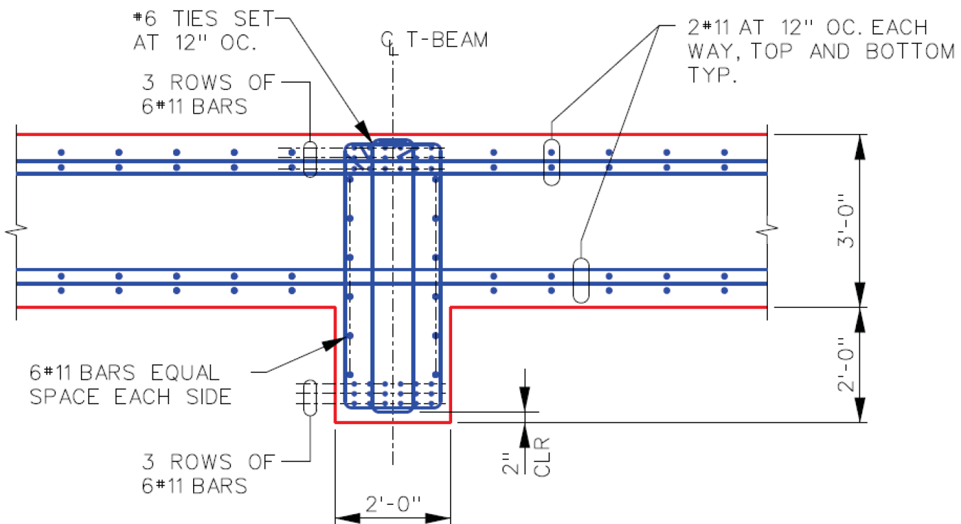
Figure 3B-39: RXB Reinforcement Detail for Type 2 T-Beams at EL 75'-0"
