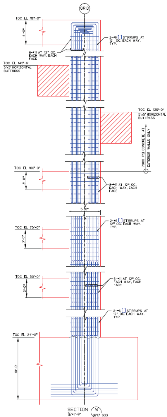
Figure 3B-9: RXB Reinforcement Section View of Wall on Grid Line 1
