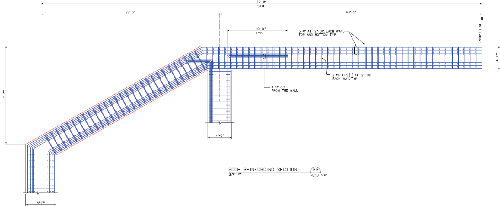
Figure 3B-30: RXB Reinforcement Section View of Roof Slab
