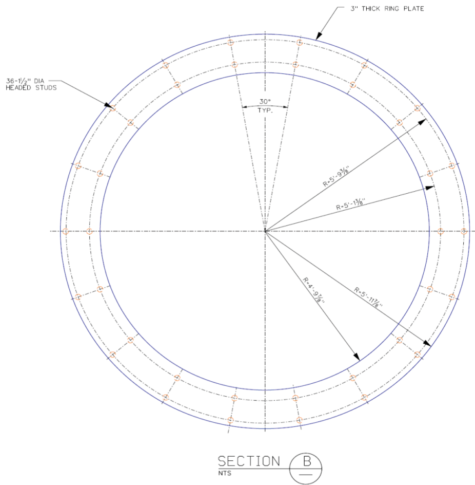
Figure 3B-50: Plan View of NPM Base Support at Bearing Ring Plate (Section B from Figure 3B-48)
