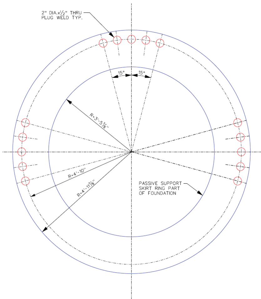
Figure 3B-49: Plan View of NPM Base Support at Passive Ring (Section A from Figure 3B-48)
