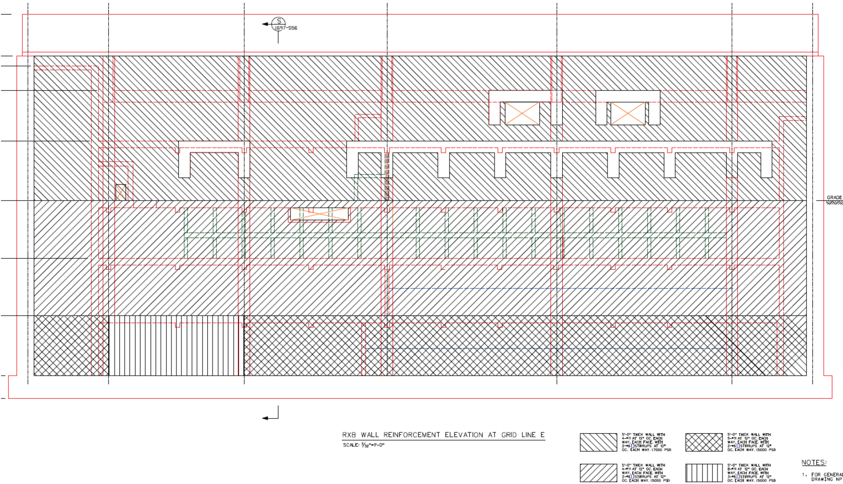
Figure 3B-23: RXB Reinforcement Elevation at Grid Line E Wall
