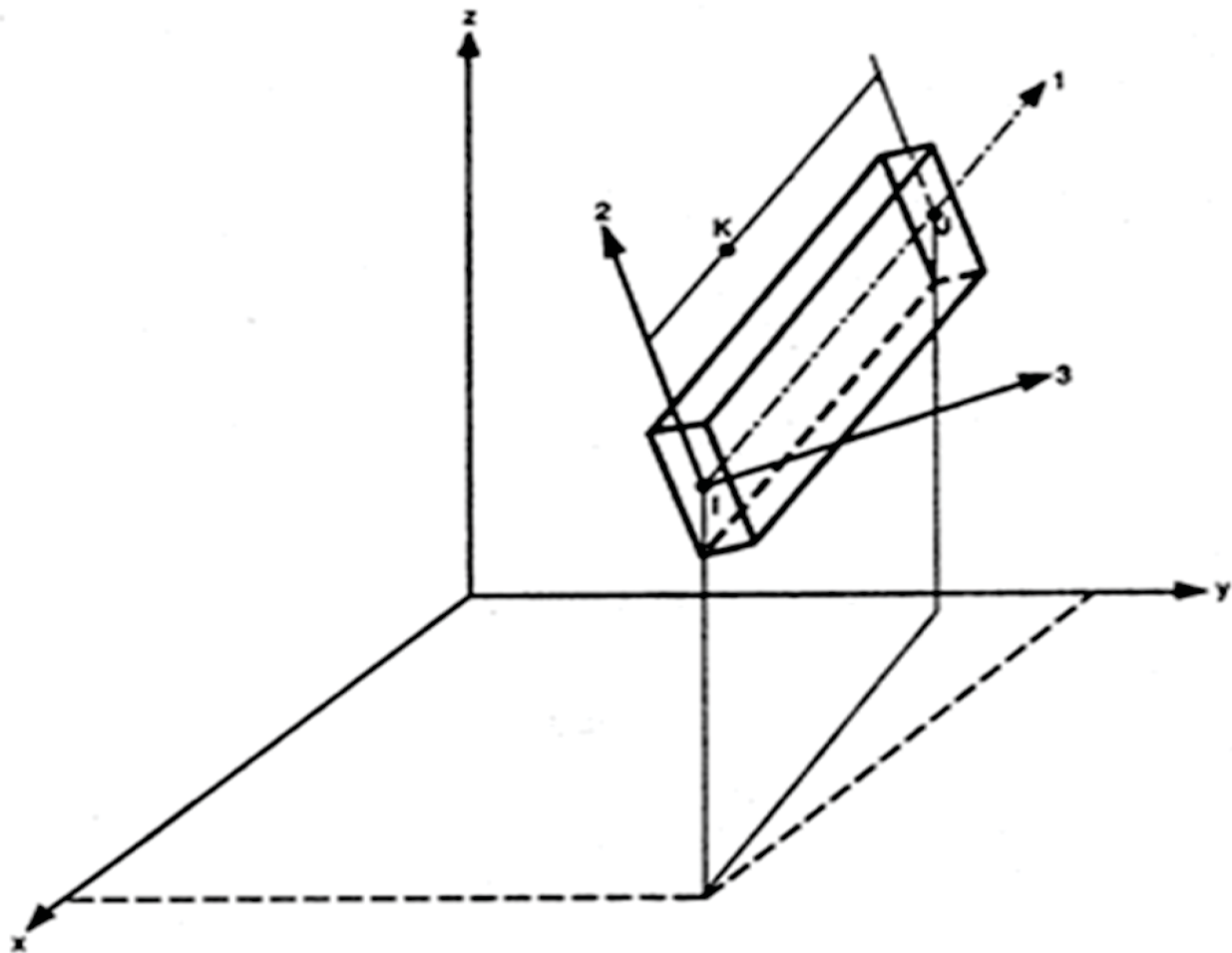
Figure 3B-6: SASSI2010 Frame Element Results Definition
