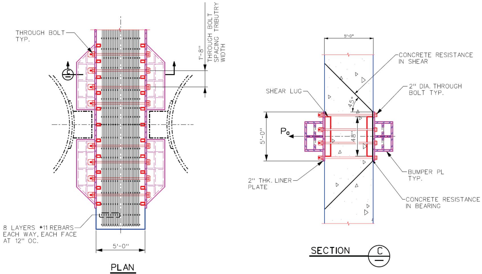
Figure 3B-64: Schematic Details of Shear Lugs and Through Bolts
