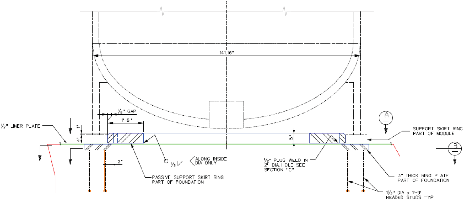
Figure 3B-48: Elevation View of the NPM Base Support at RXB Pool Floor
