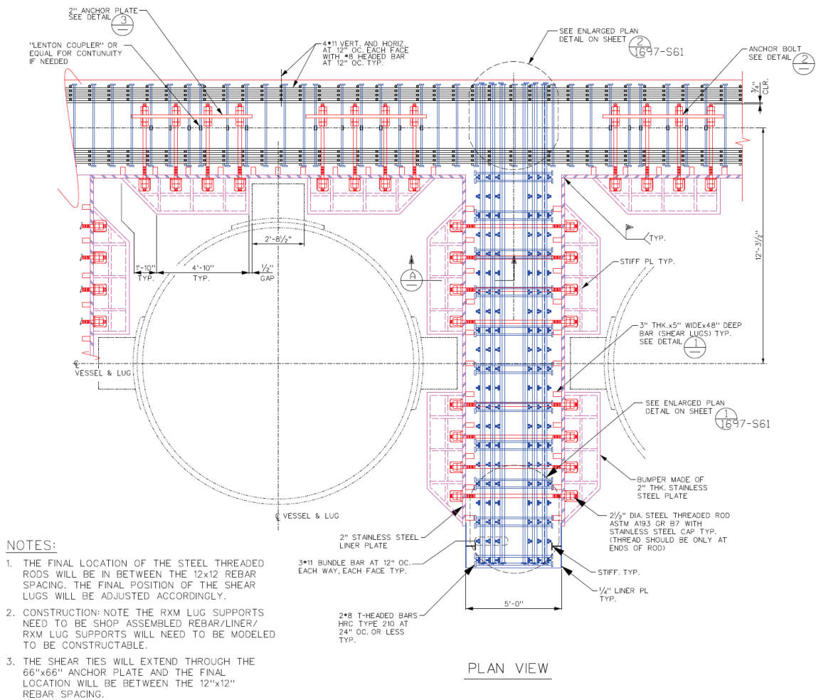
Figure 3B-51: NPM Lug Support Plan View and Details
