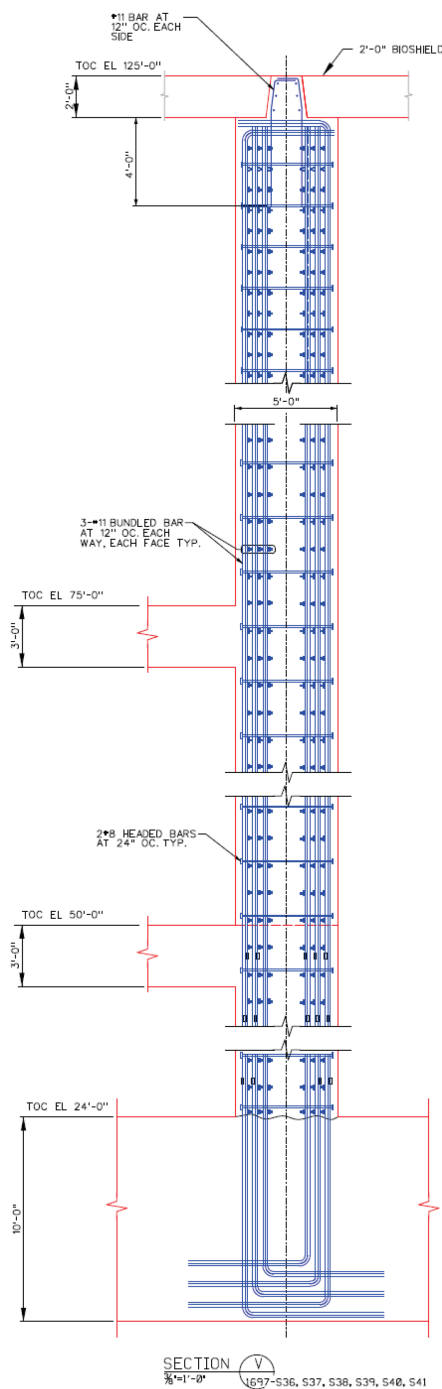
Figure 3B-44: RXB Reinforcement Section View of 5 Foot Thick Wall on RXB Grid Line 4
