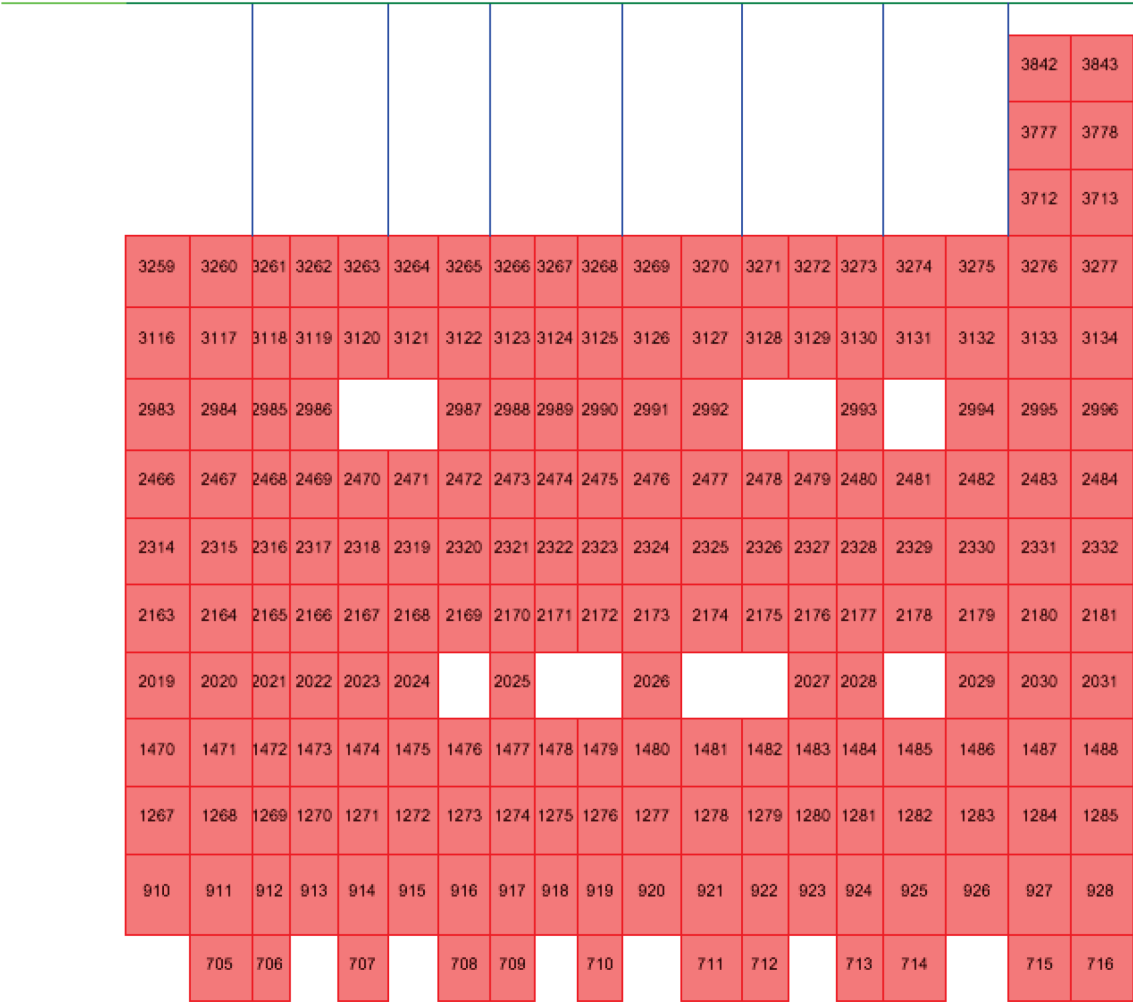
Figure 3B-65: SAP2000 Elevation View and Shell Element Numbers at CRB Grid Line 3 (Looking North)
