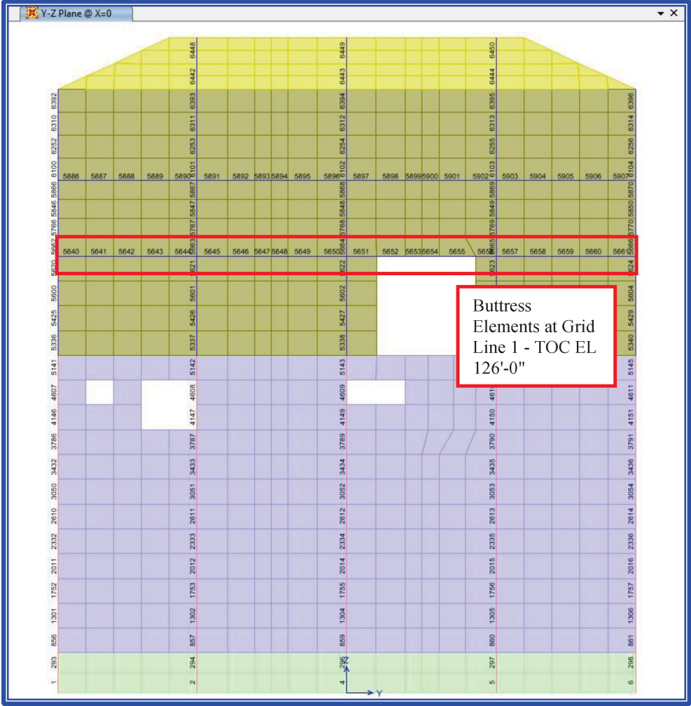
Figure 3B-40: SAP2000 View and Frame Element Numbers of Buttresses at Grid Line 1 on RXB EL. 126'-0"
