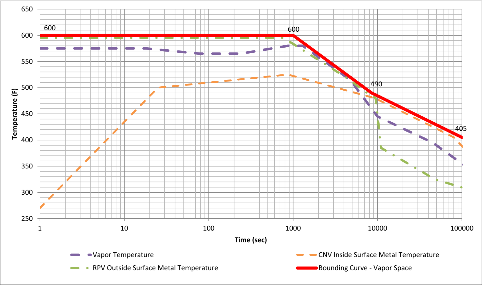
Figure 3C-2: Containment Vapor Space Metal and Gas Temperatures with Bounding Curve (Zones C, D, E, and F)
