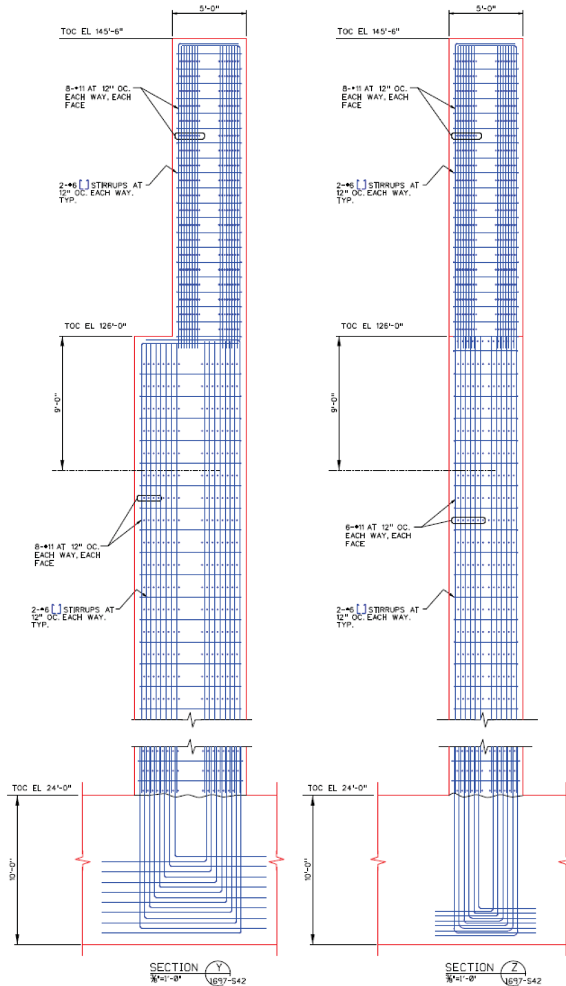
Figure 3B-21: RXB Reinforcement Section Views of Pool Wall on Grid Line 6
