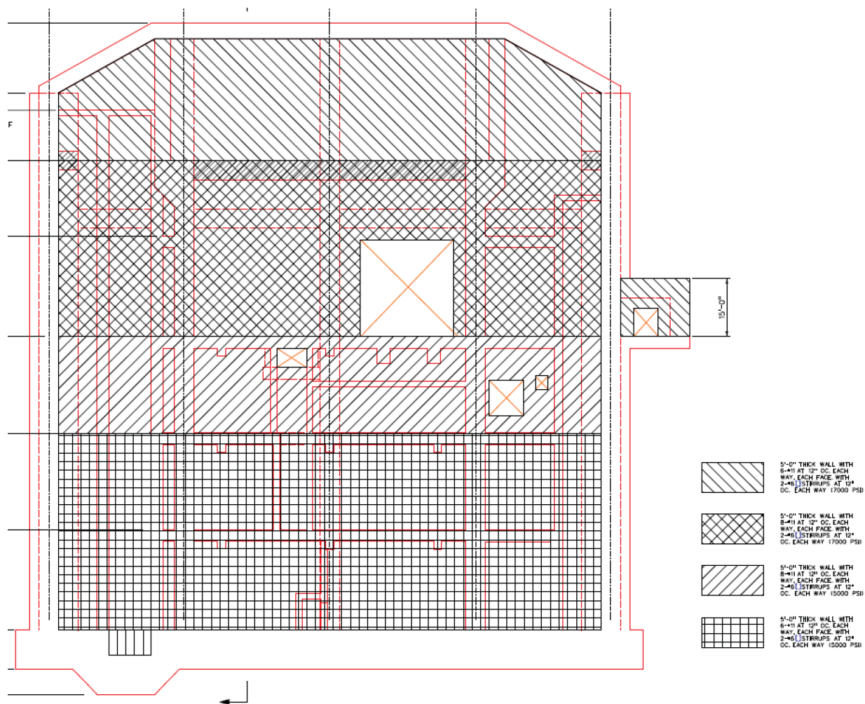
Figure 3B-8: RXB Reinforcement Elevation at Grid Line 1 Wall
