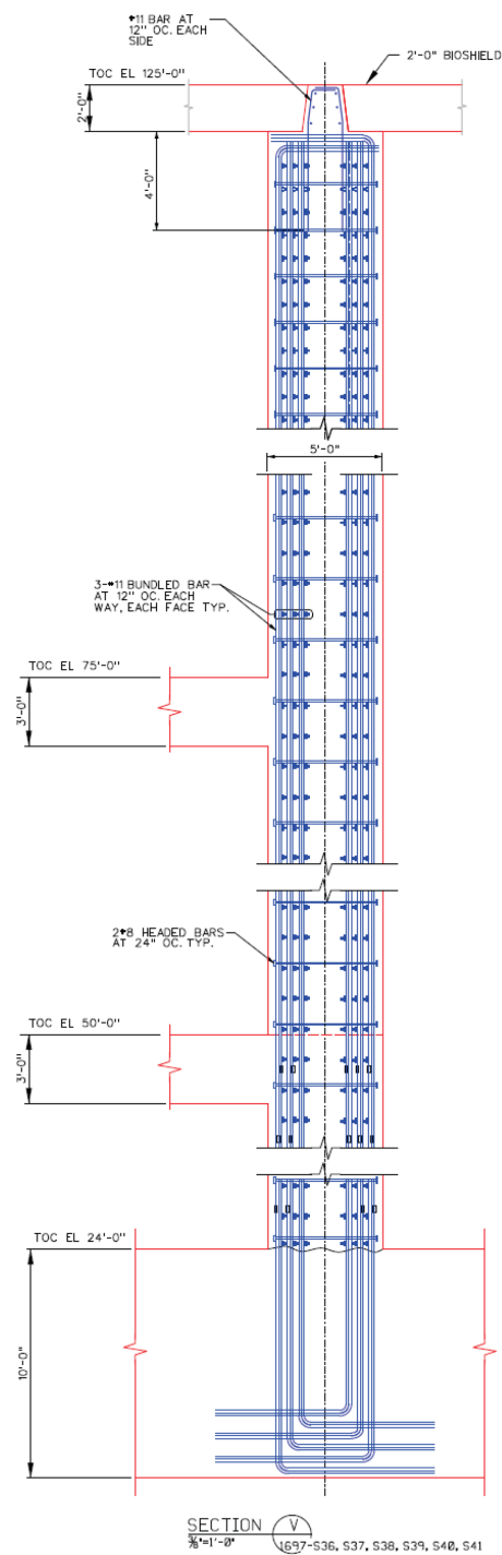
Figure 3B-16: RXB Reinforcement Section View of 5 ft Thick Wall on Grid Line 4
