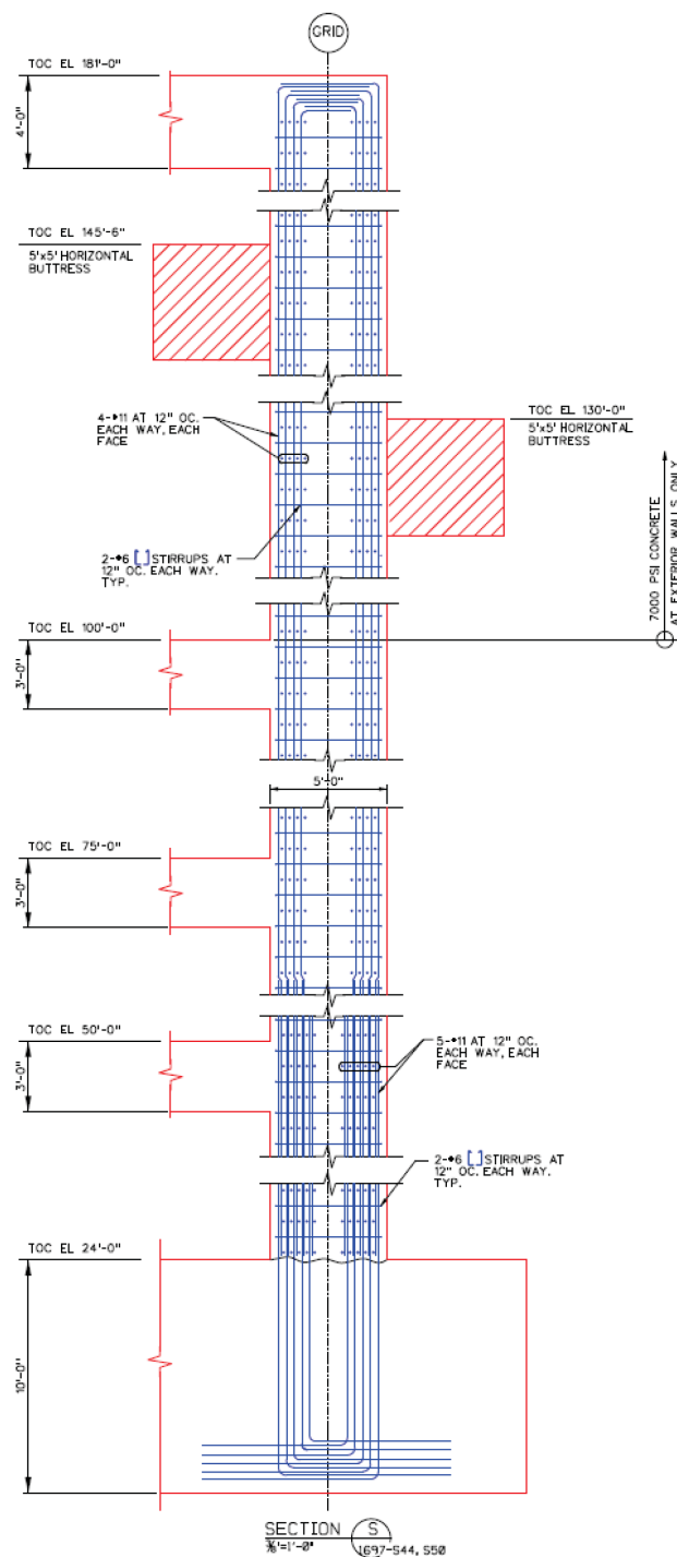
Figure 3B-24: RXB Reinforcement Section View of Wall on Grid Line E
