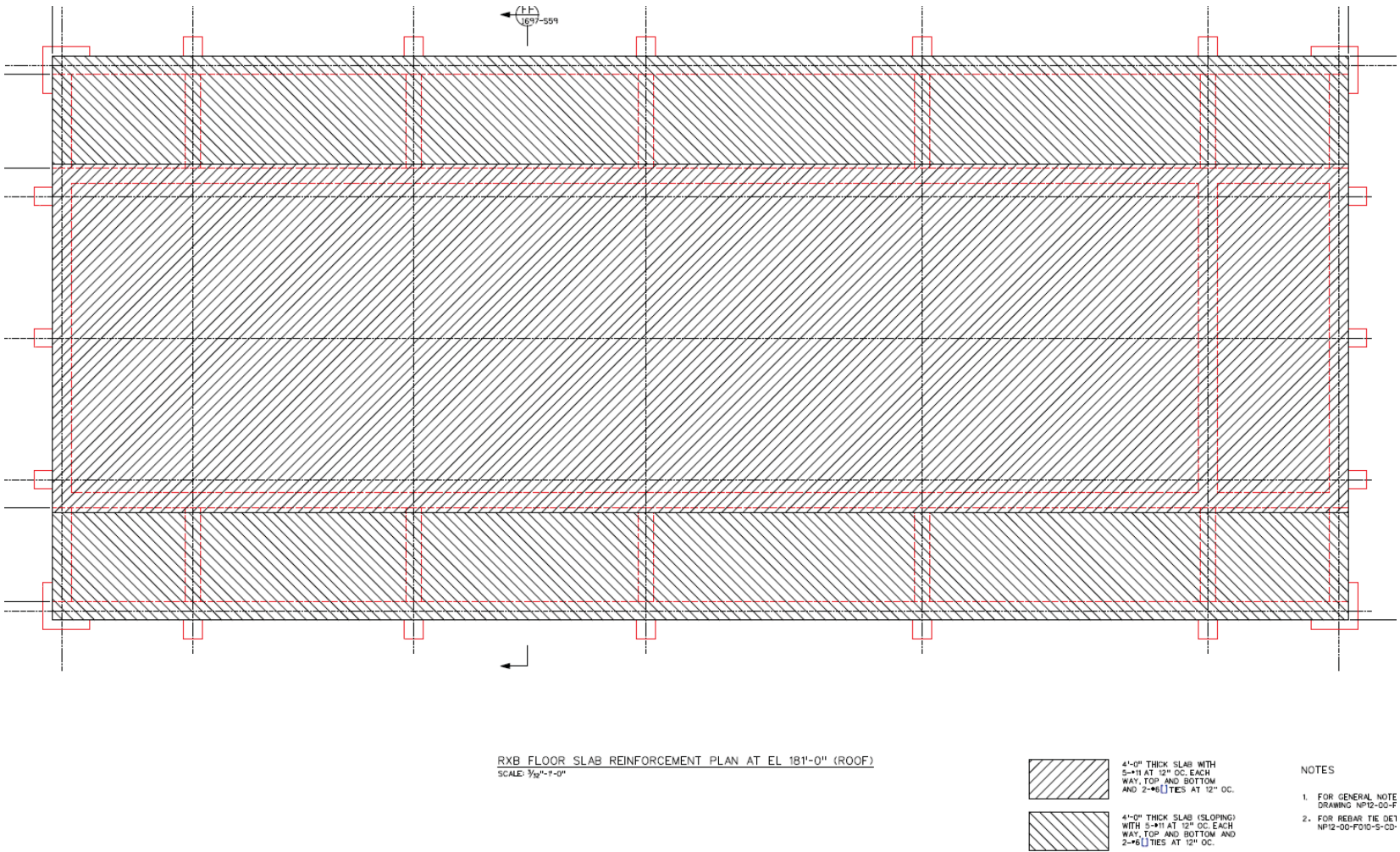
Figure 3B-29: RXB Reinforcement Plan for Roof Slab
