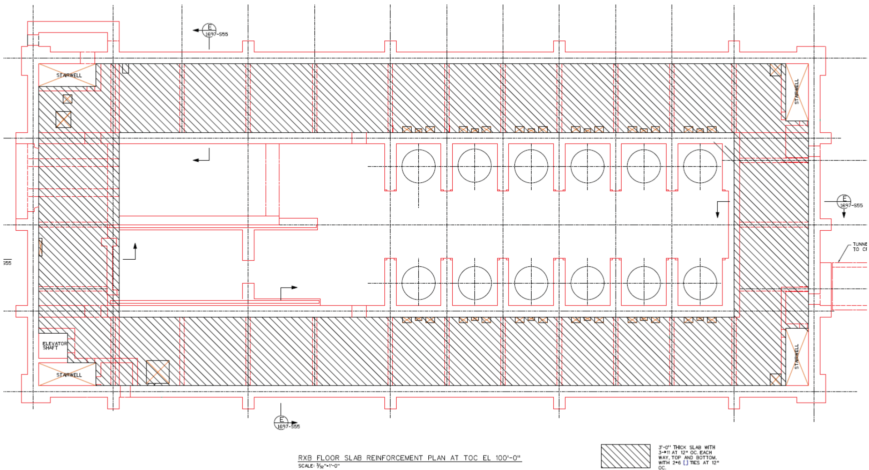
Figure 3B-26: RXB Reinforcement Plan at EL 100'-0"
