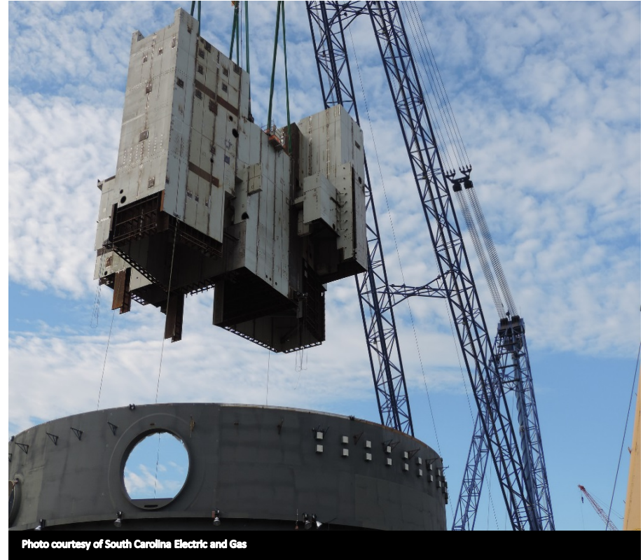
V.C. Summer – Steam Generator & Refueling Canal Module Placement
