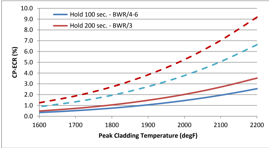
Figure 3.1: Calculated Oxidation (CP-ECR versus Temperature) (solid line – no burst, dotted line – burst)
