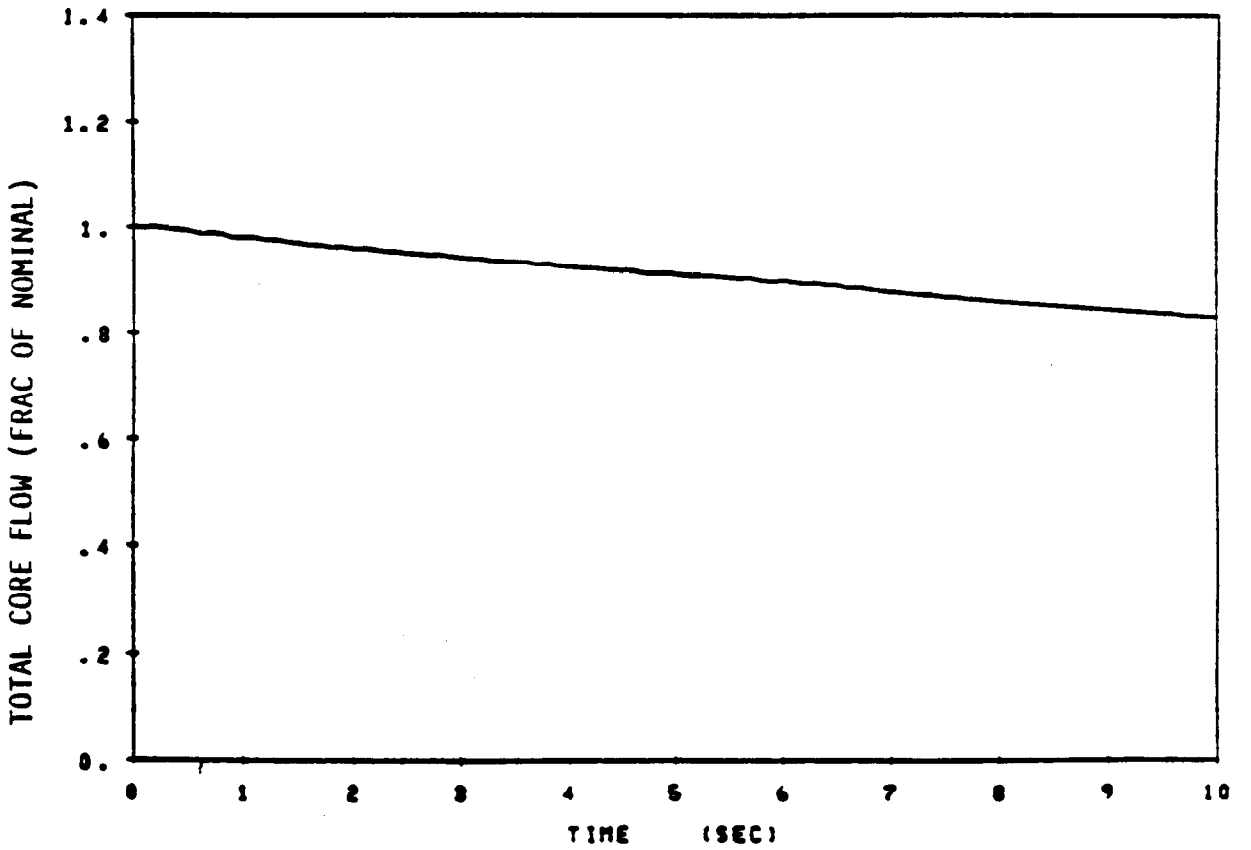
Figure 14.1.6-5 Partial Loss of Flow 1/4 Faulted Loop and Core Flows Versus Time
