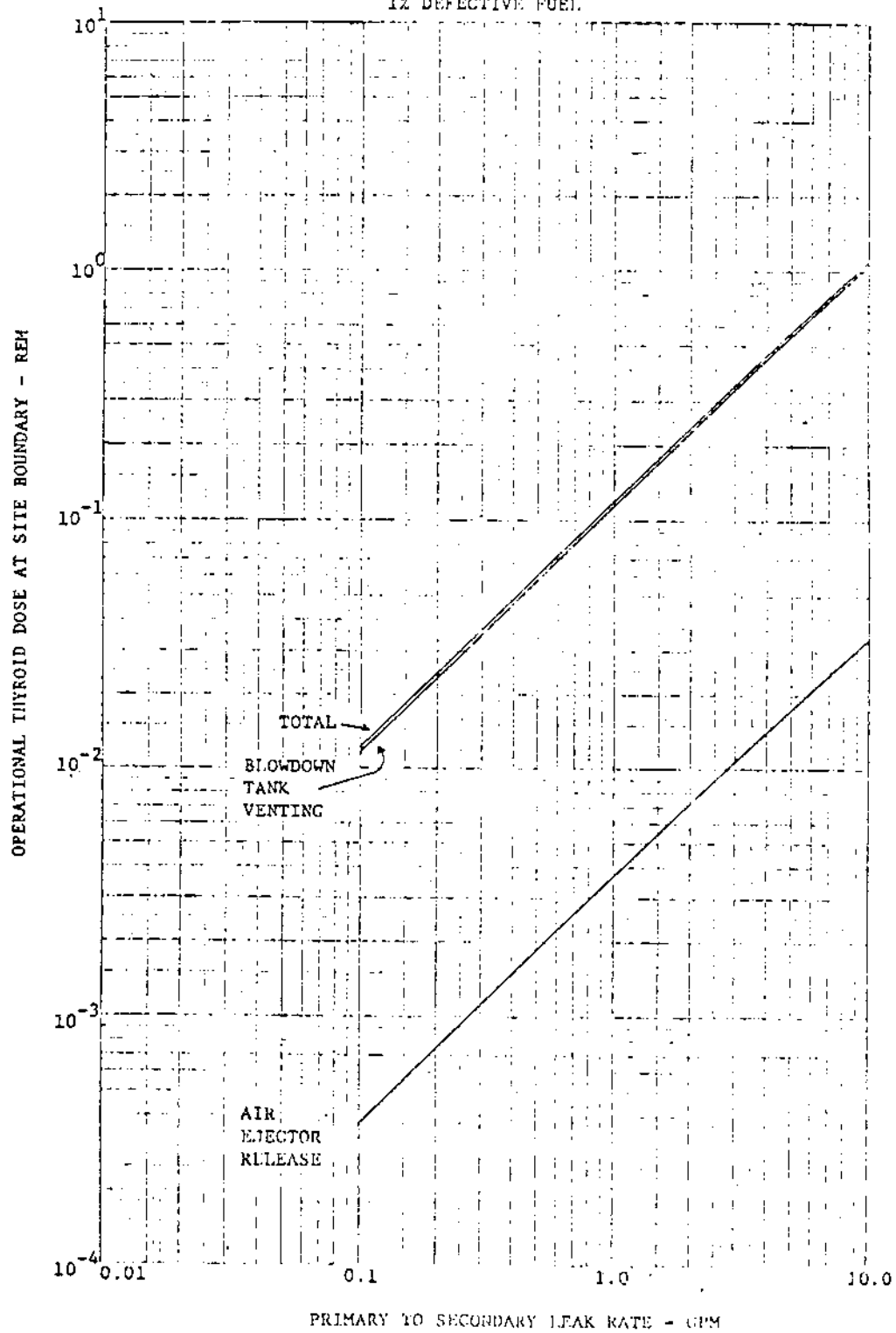
FIGURE 14.2.7-1 ANNUAL OPERATIONAL THYROID DOSES AT SITE BOUNDARY 1% DEFECTIVE FUEL
