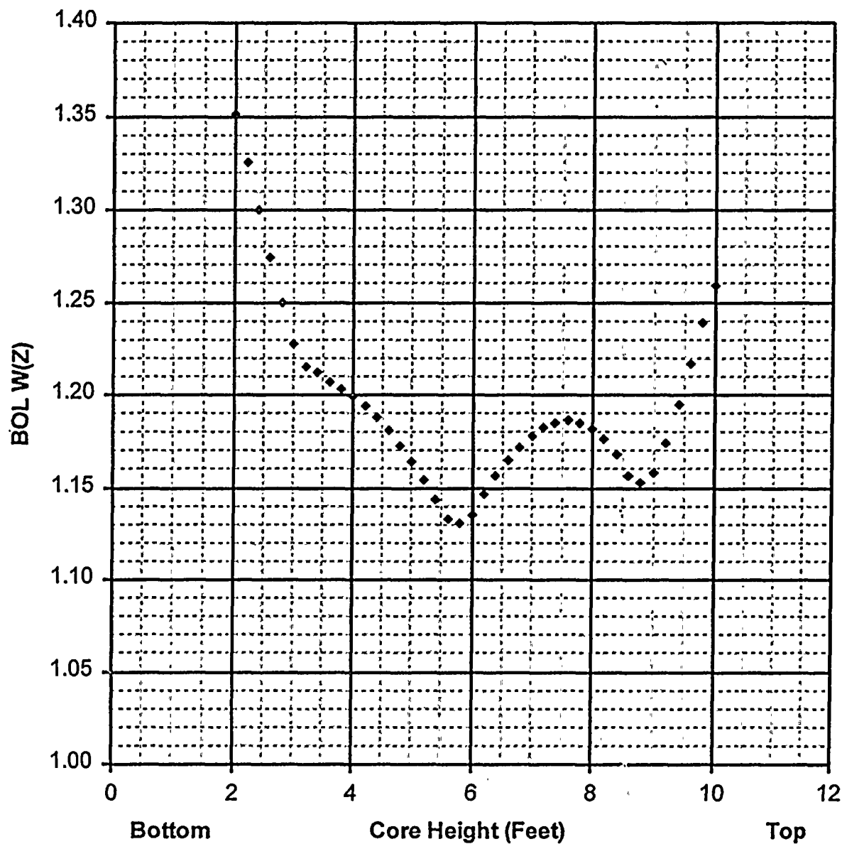
Figure 3 Load Follow W(Z) at 150 MWD/MTU as a Function of Core Height * Top and Bottom 15% Excluded Per Tech Spec 4.2.2.2.g
