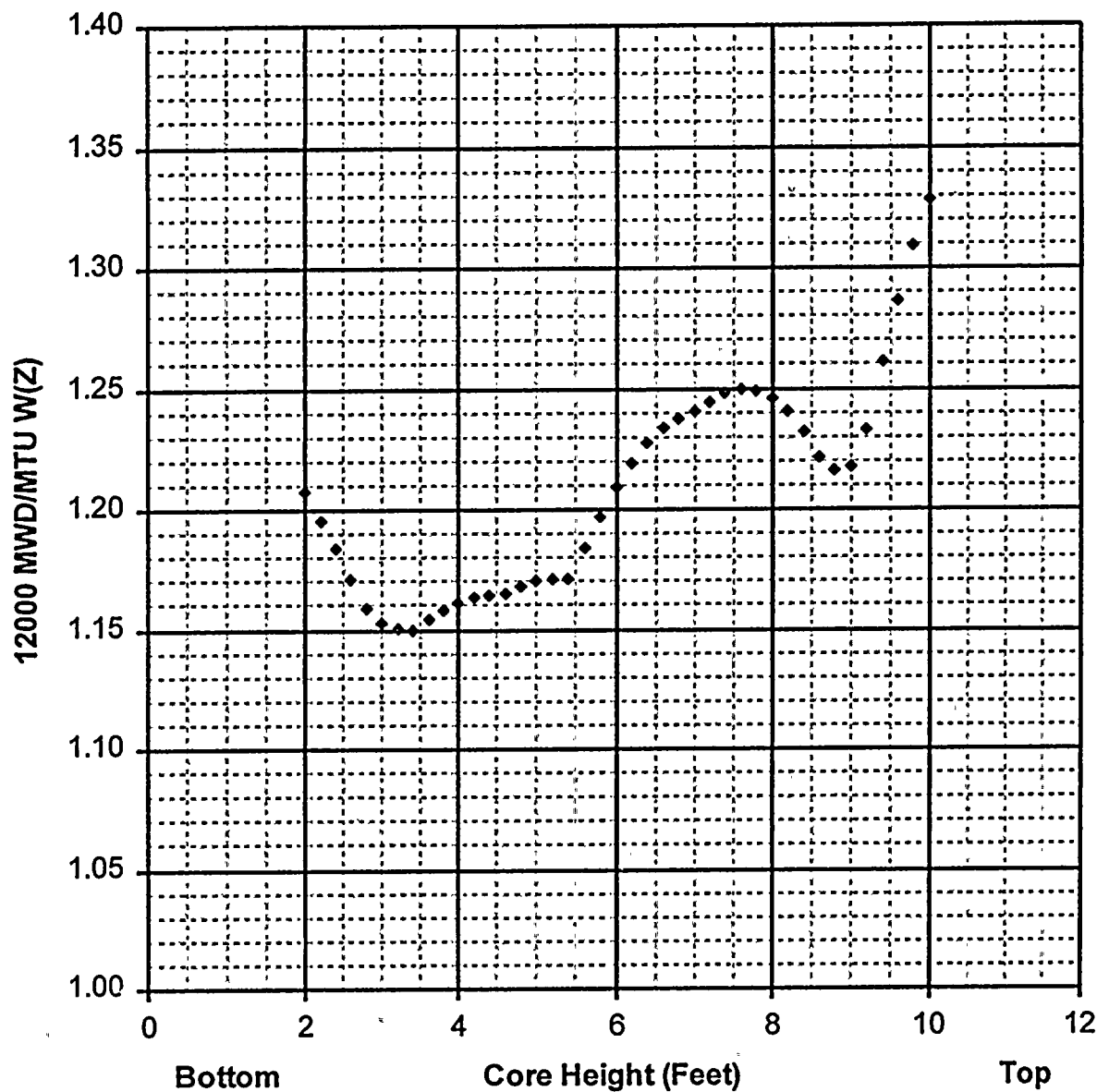
Figure 5 Load Follow W(Z) at 12000 MWD/MTU as a Function of Core Height * Top and Bottom 15% Excluded Per Tech Spec 4.2.2.2.g
