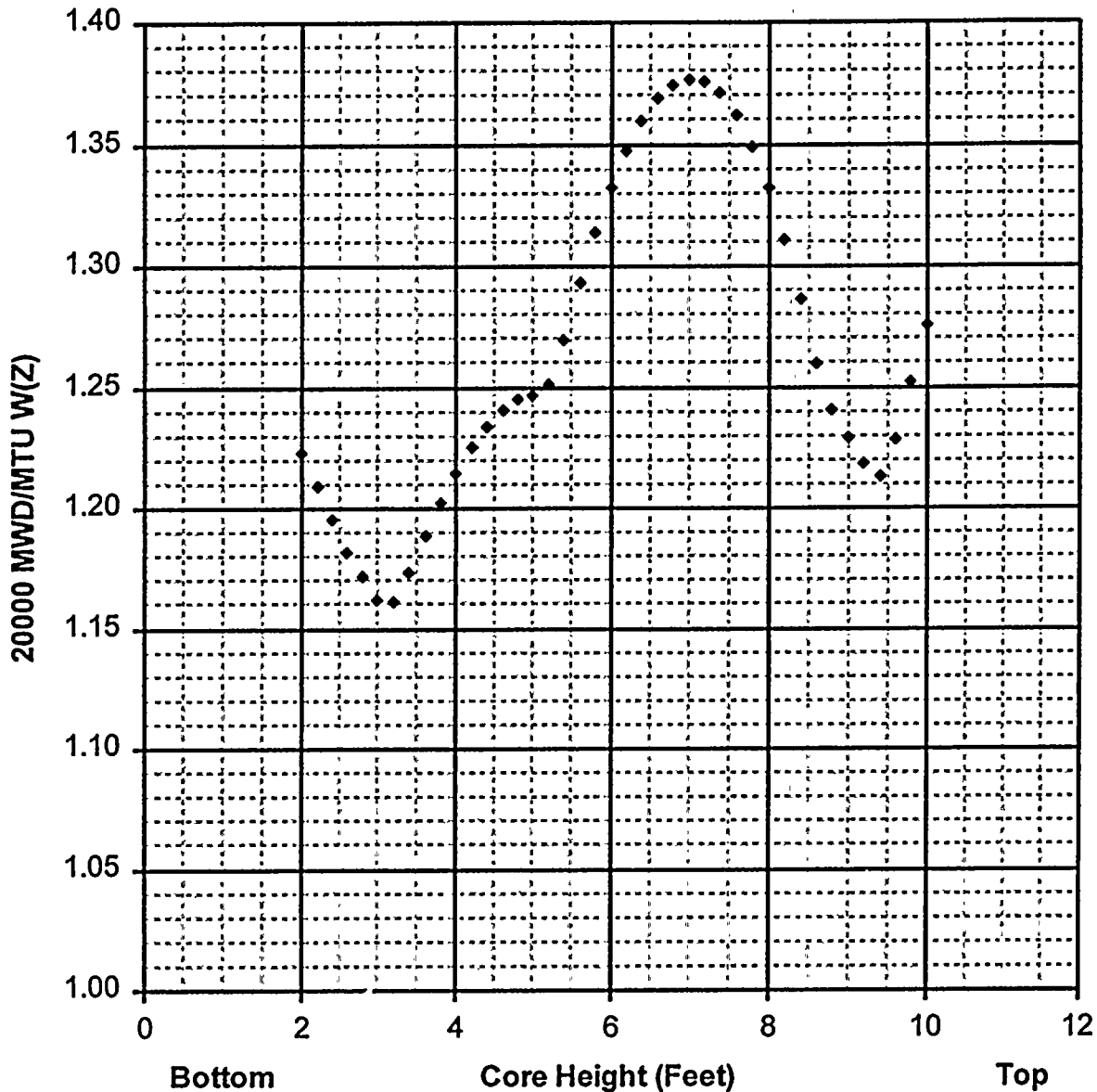
Figure 6 Load Follow W(Z) at 20000 MWD/MTU as a Function of Core Height * Top and Bottom 15% Excluded Per Tech Spec 4.2.2.2.g
