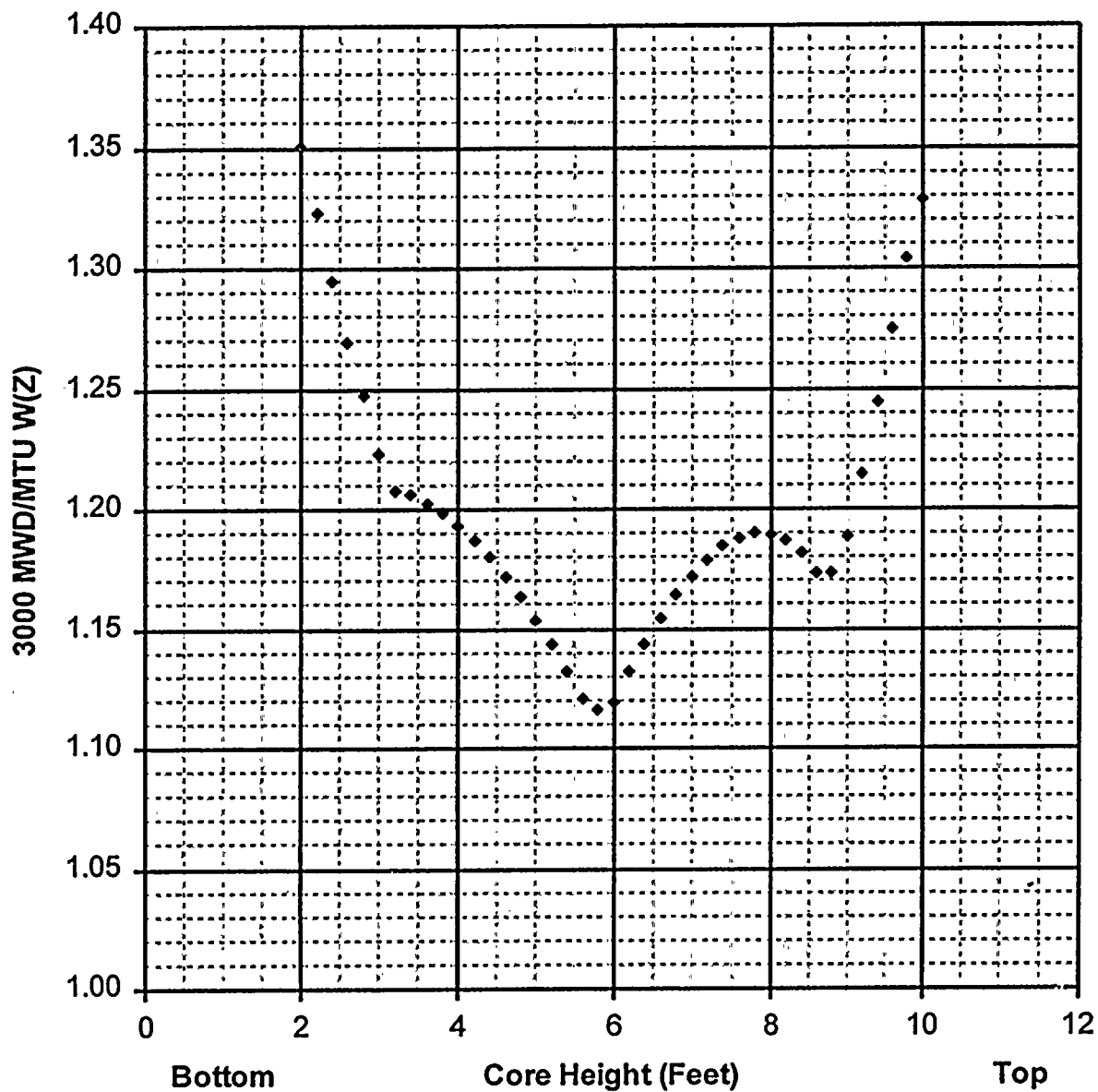
Figure 4 Load Follow W(Z) at 3000 MWD/MTU as a Function of Core Height *Top and Bottom 15% Excluded Per Tech Spec 4.2.2.2.g
