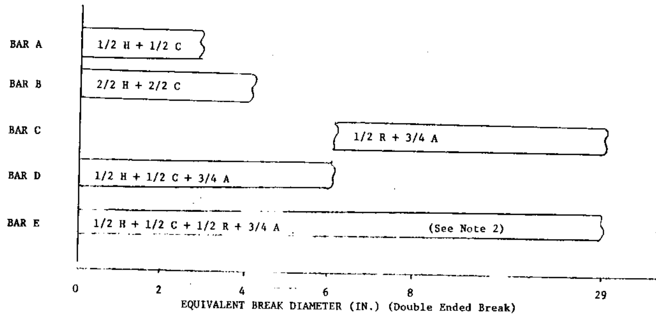
RANGE OF CORE PROTECTION PROVIDED BY VARIOUS COMPONENTS OF THE EMERGENCY CORE COOLING SYSTEM
