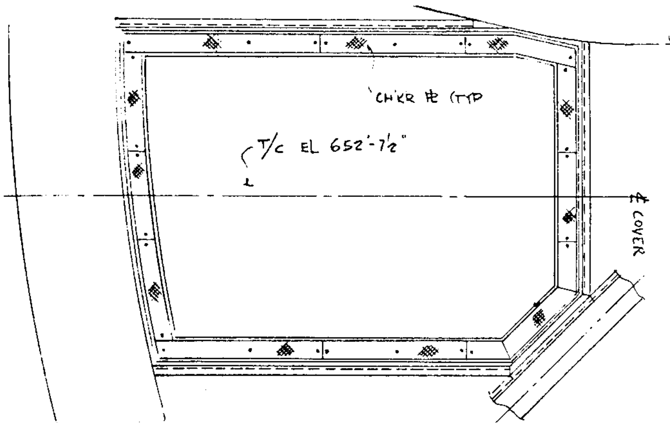
TYPICAL COVER WITH CONCRETE
