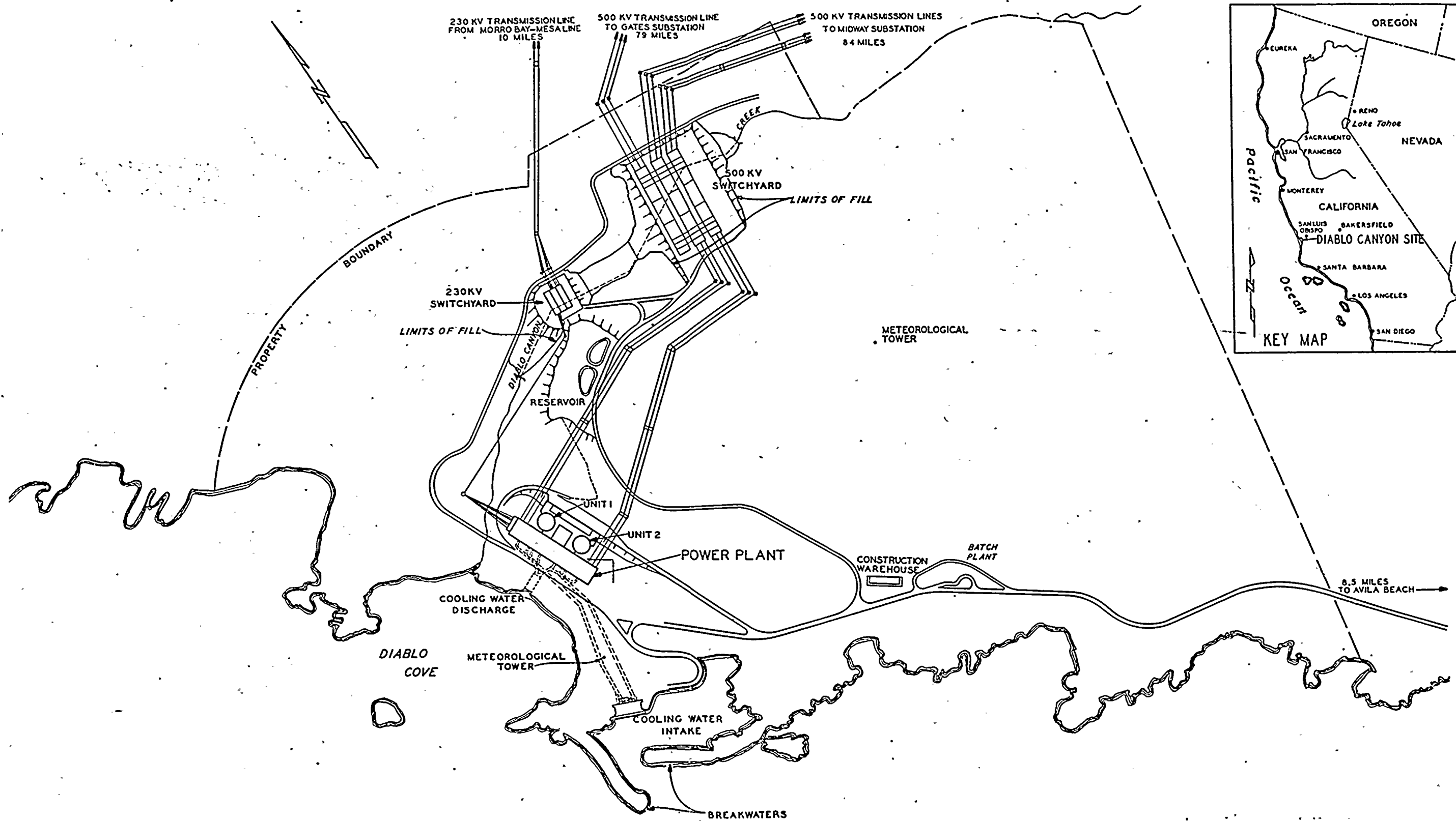
UNITS 1 AND 2 DIABLO CANYON SITE FIGURE 1.2-1 PLOT PLAN
