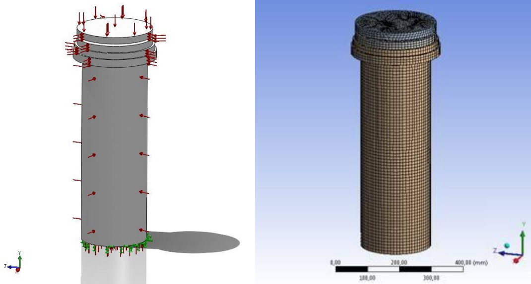
Figure 8: Status of the load and meshing of the internal assembly
