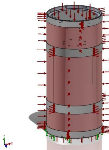
Figure 2: External view of the package
