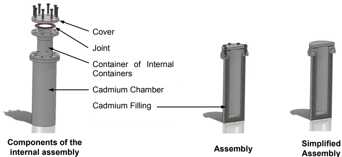
Figure 7: Components of the internal assembly
