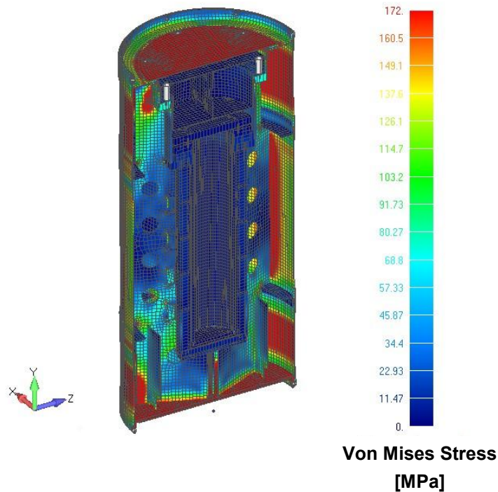
Figure 6: Stresses in the package subject to external pressure
