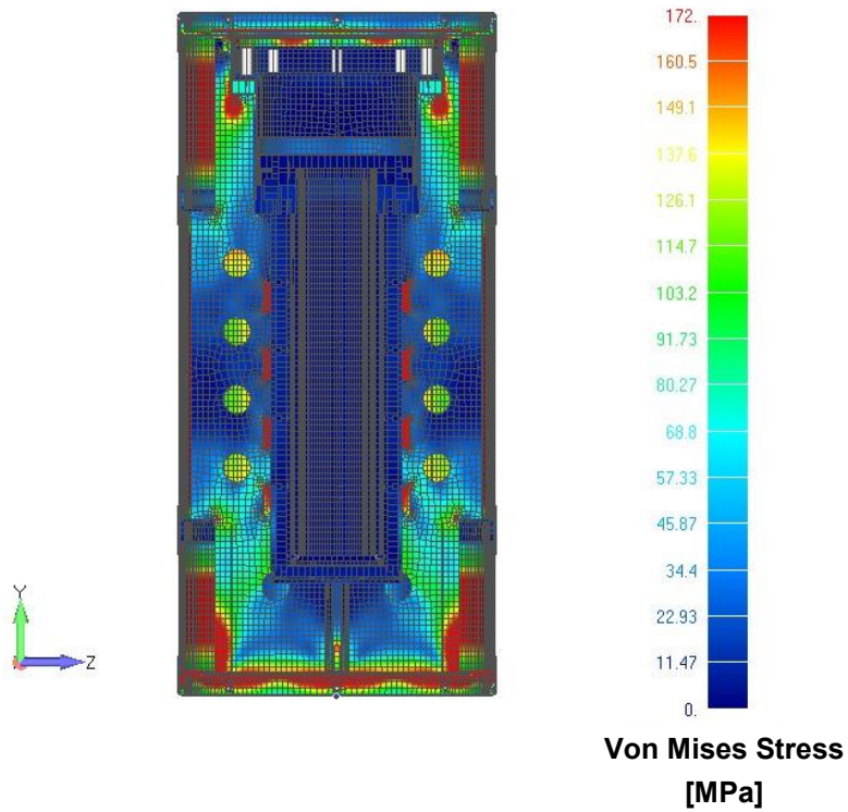
Figure 5: (Internal) Stresses in the package subject to external pressure
