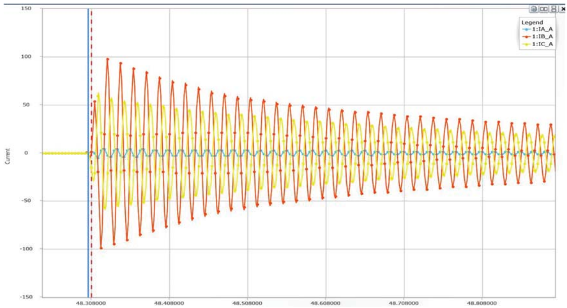
Figure 3: Event report from field on transformer inrush
