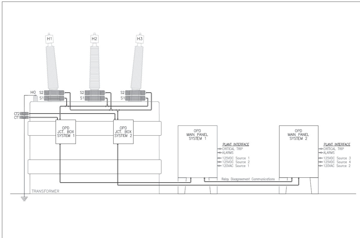
System Layout Drawing
