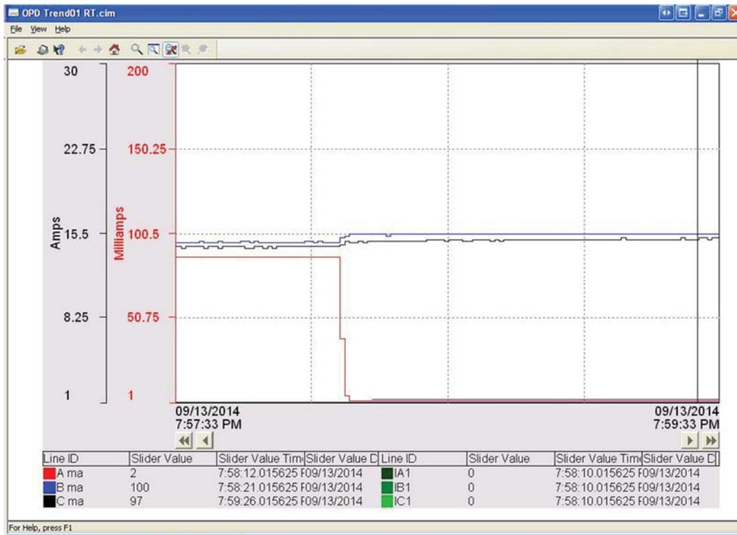
Figure 6: Lab data from "A"-phase open test case.
