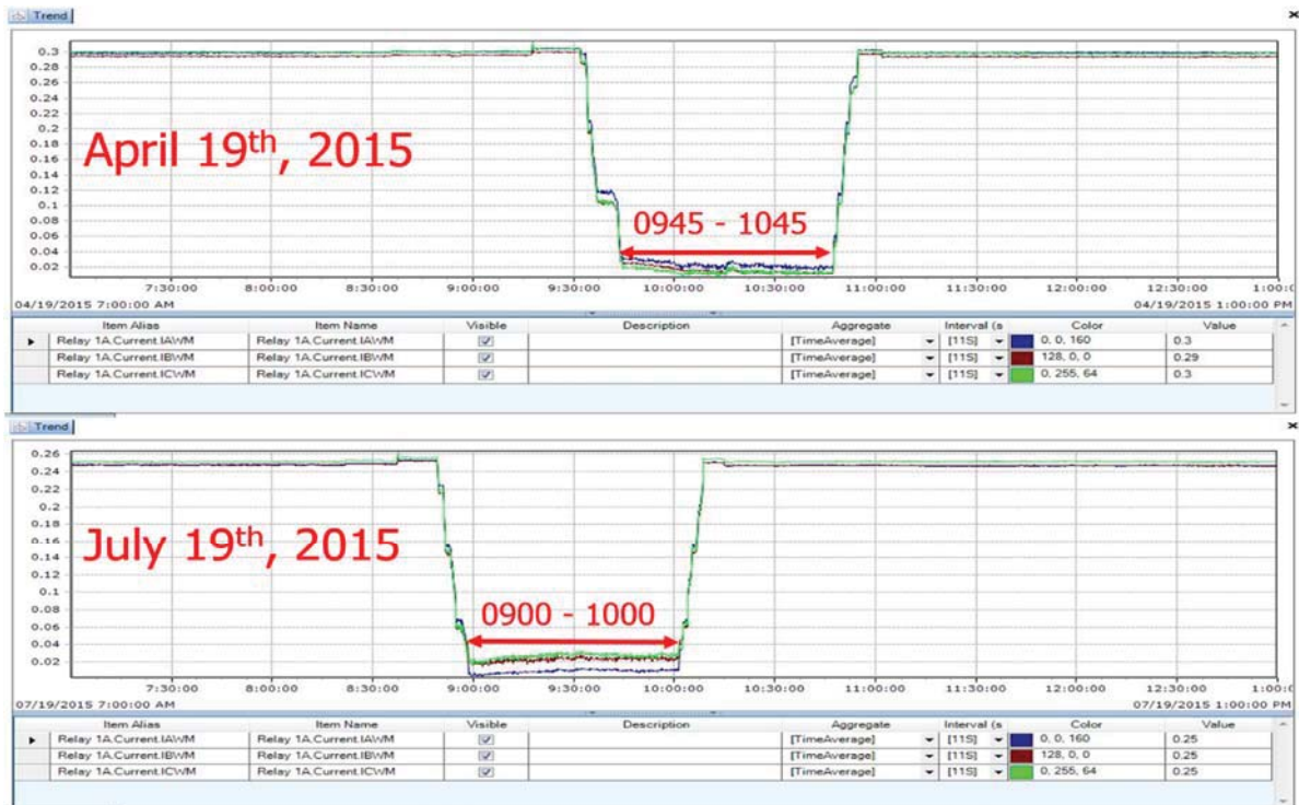
Figure 2: Field data on diesel surveillance pattern 60-minute outage every mid-month between 0800 and 1200 Vertical axis per unit load current on transformer
