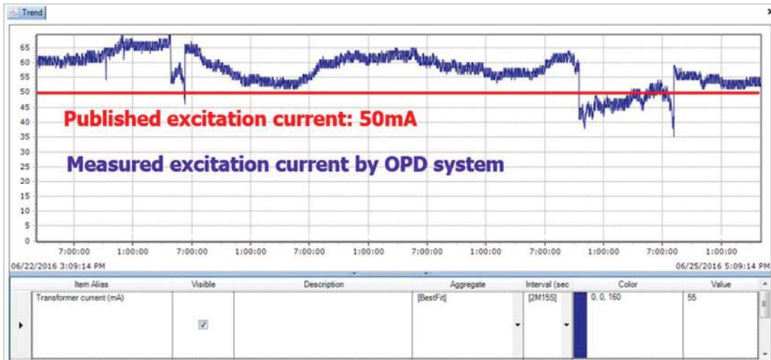
Figure 1: Field data on 345kV transformer exciting current (3 \phi avg.) Field data vs. published data
