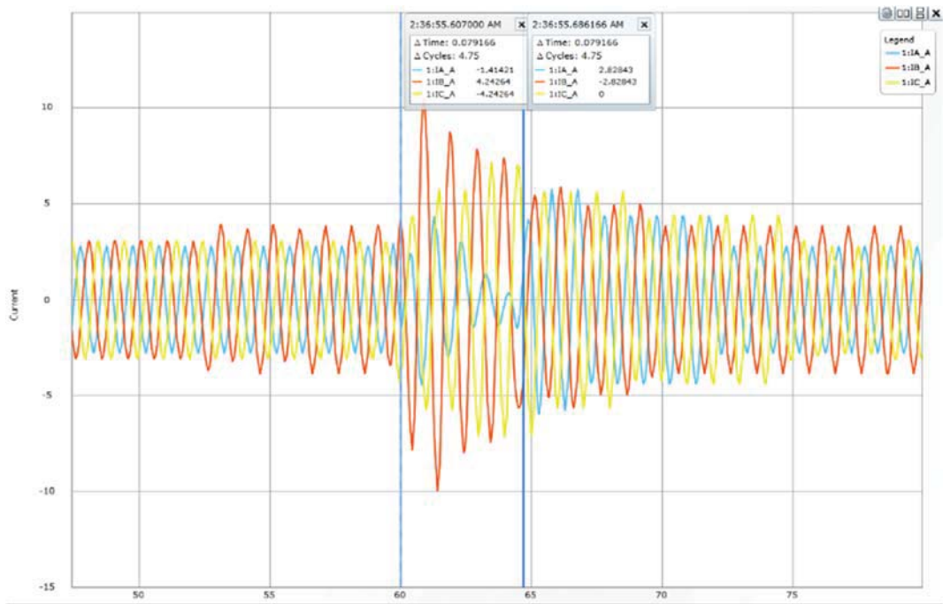
Figure 5: Event report from field on 230kV phase-phase fault
