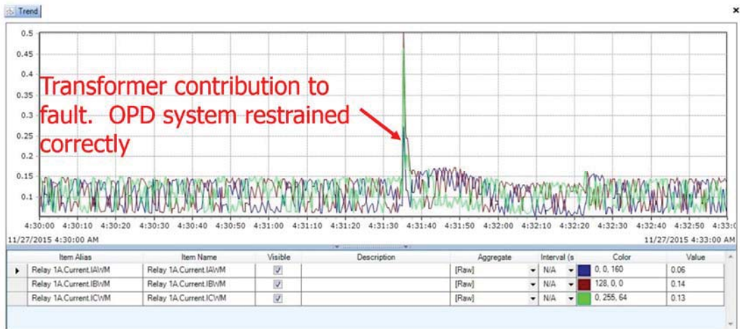
Figure 4: Trend data from field on 230kV ground fault Vertical axis per unit load current on transformer
