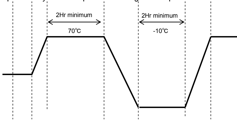
Figure 5-7 Temperature and Humidity Profile for Temperature Cycle Test
