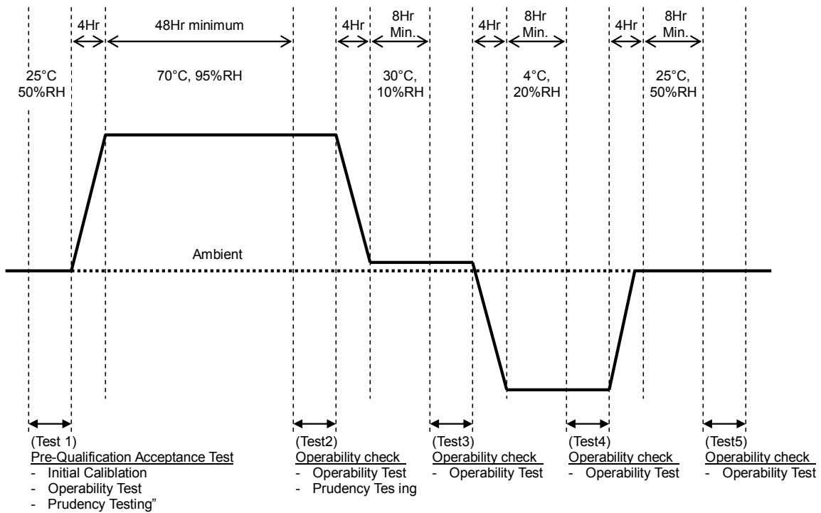
Figure 5-8 Temperature and Humidity Profile
