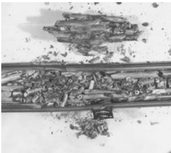
Figure 1. Section of the FLECHT Run 9573 Test Bundle that Incurred Runaway Oxidation
