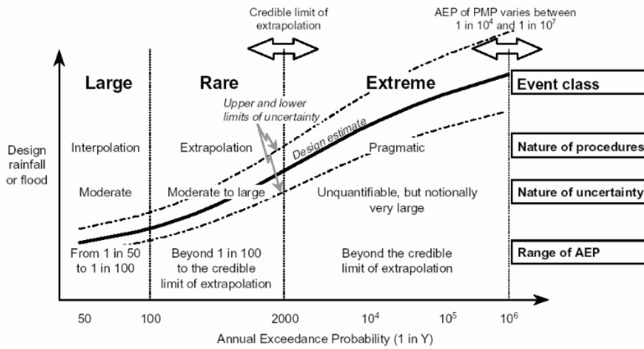
Figure Error! No text of specified style in document.-1: Characteristics of Notional Floods (Nathan and Weinmann, 2001)
