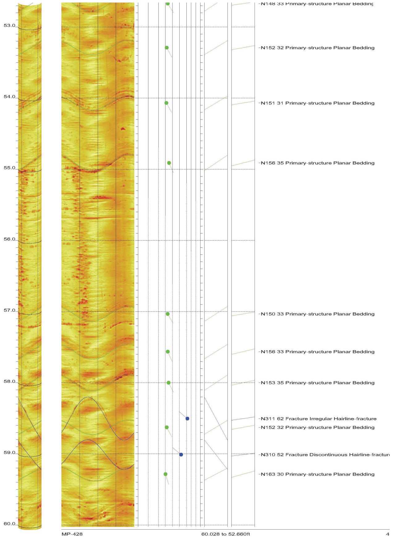
AMEC Clinch River SMR Project Borehole MP-428 Acoustic Televiewer Features rev 2 Sheet 4 of 30
