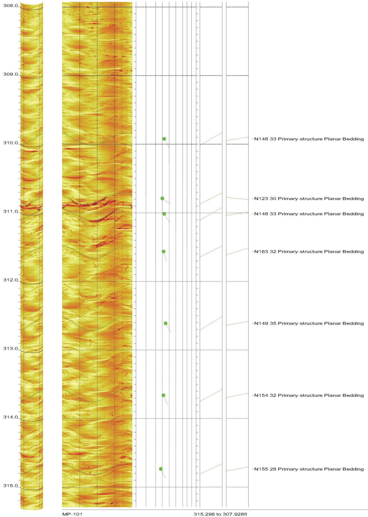
AMEC Clinch River SMR Project Borehole MP-101 Acoustic Televiewer Features rev 2 Sheet 41 of 72
