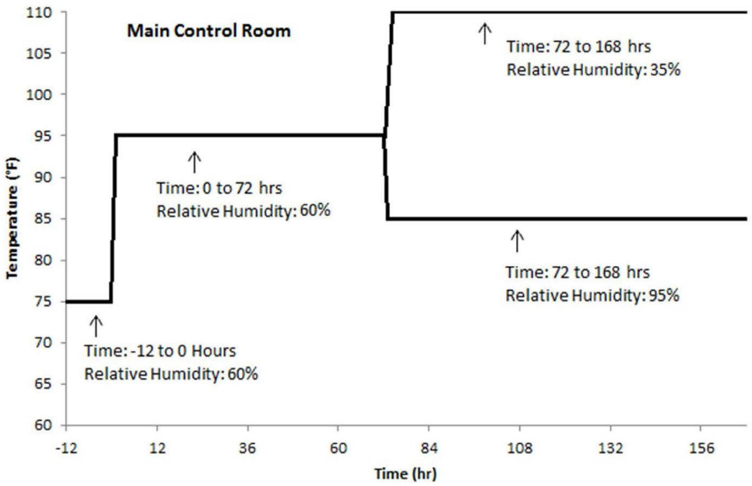
WILLIAM STATES LEE III NUCLEAR STATION UNITS 1 & 2 TYPICAL ABNORMAL ENVIRONMENTAL TEST PROFILE: MAIN CONTROL ROOM FIGURE 3D-201 Rev 11
