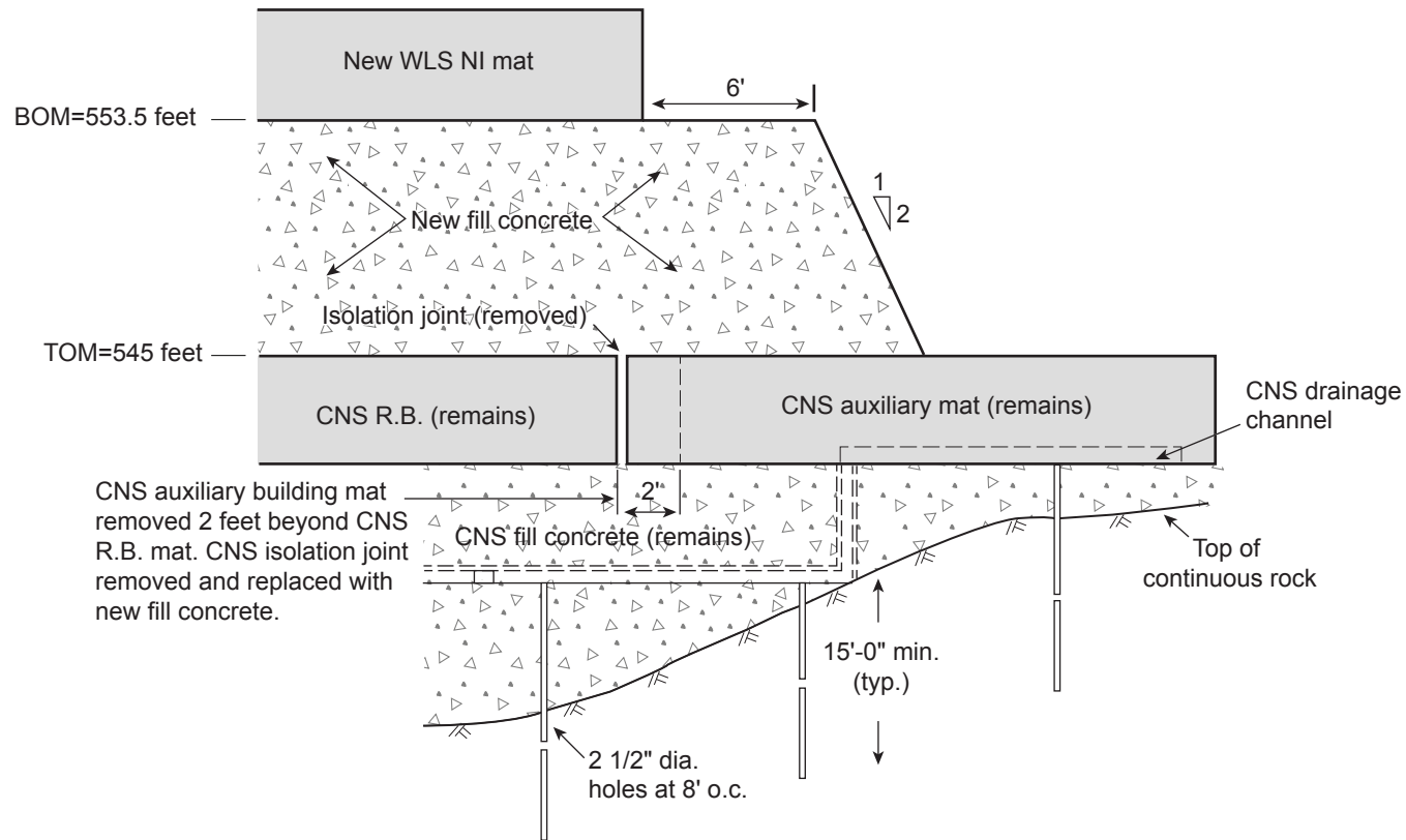
DETAIL 2
