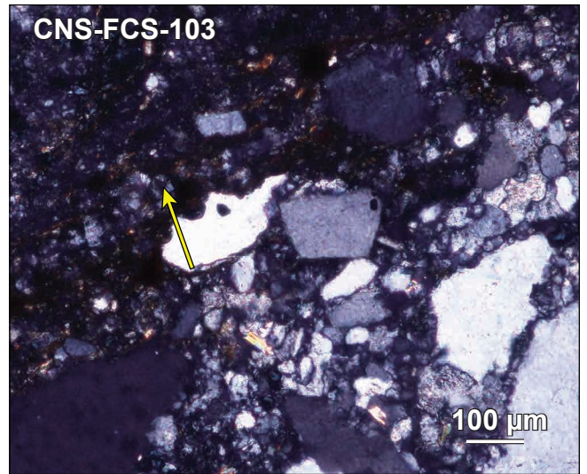
Photomicrograph thin section CNS-FC8-103. Low birefringent material [K-feldspar, Adularia (?)] in veins cross cutting structural fabric indicated by yellow arrow (left image - plain light, right image - cross-polarized light).
