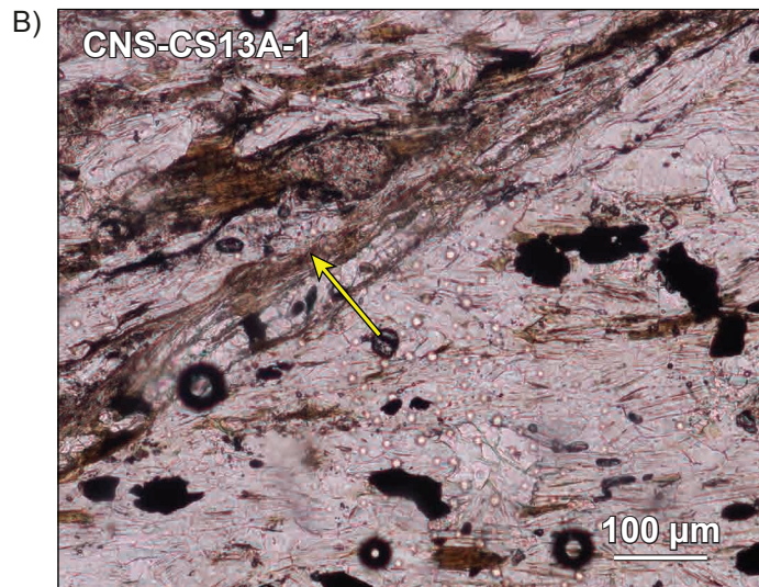
Photomicrograph thin section CNS-CS13A-1, low birefringent material [K-feldspar, Adularia (?)] in veins cross cutting structural fabric indicated by yellow arrow (left image - plain light, right image - cross-polarized light).
