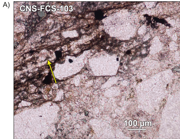
Photomicrograph thin section CNS-FC8-103. Low birefringent material [K-feldspar, Adularia (?)] in veins cross cutting structural fabric indicated by yellow arrow (left image - plain light, right image - cross-polarized light).
