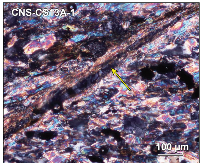
Photomicrograph thin section CNS-CS13A-1, low birefringent material [K-feldspar, Adularia (?)] in veins cross cutting structural fabric indicated by yellow arrow (left image - plain light, right image - cross-polarized light).
