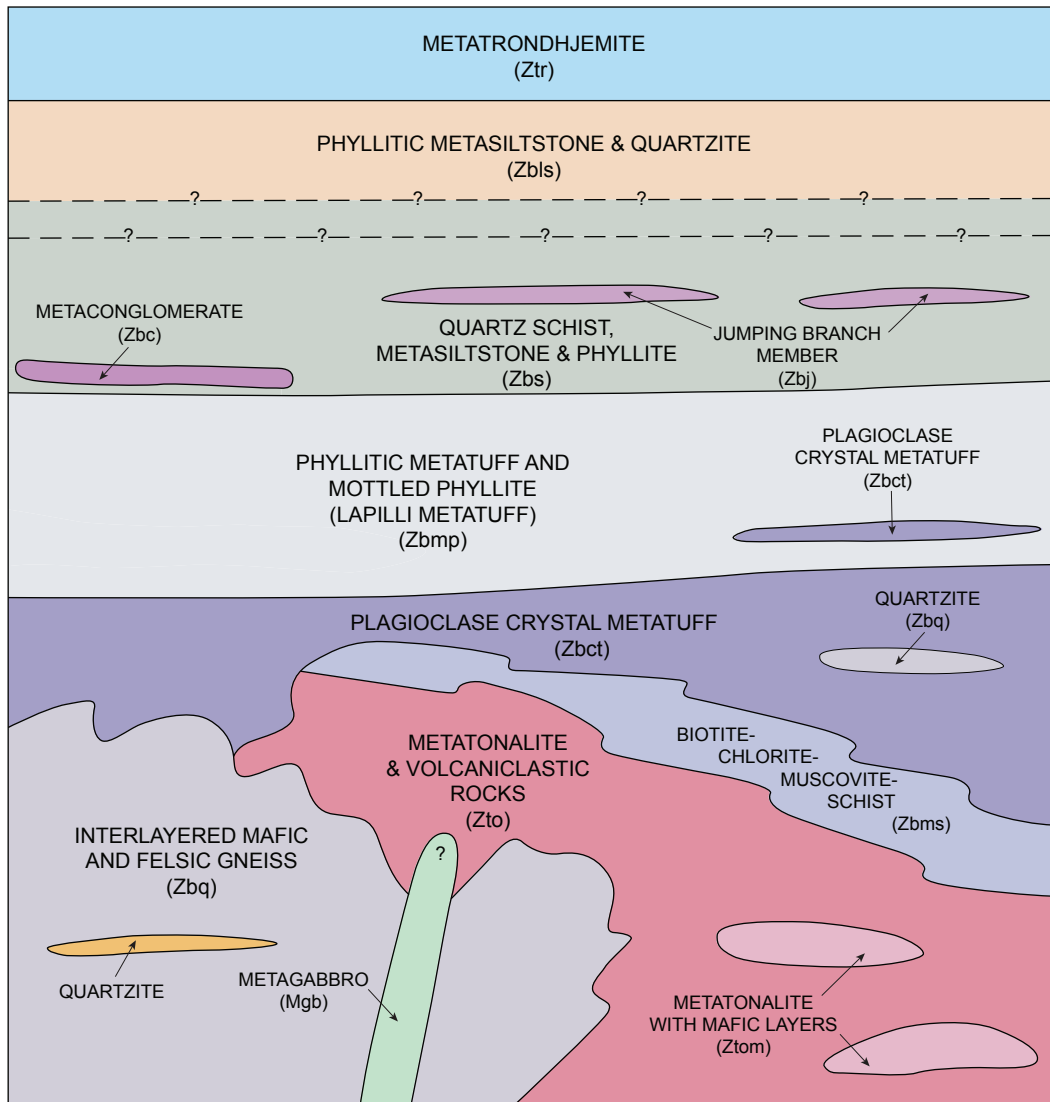
Schematic diagram of stratigraphic relations in Kings Mountain sequence prior to earliest deformation.
