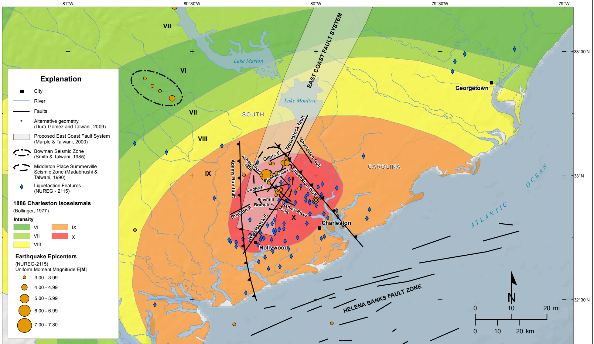
WILLIAM STATES LEE III NUCLEAR STATION UNITS 1 & 2 Local Charleston Tectonic Features FIGURE 2.5.1-216 Rev 8
