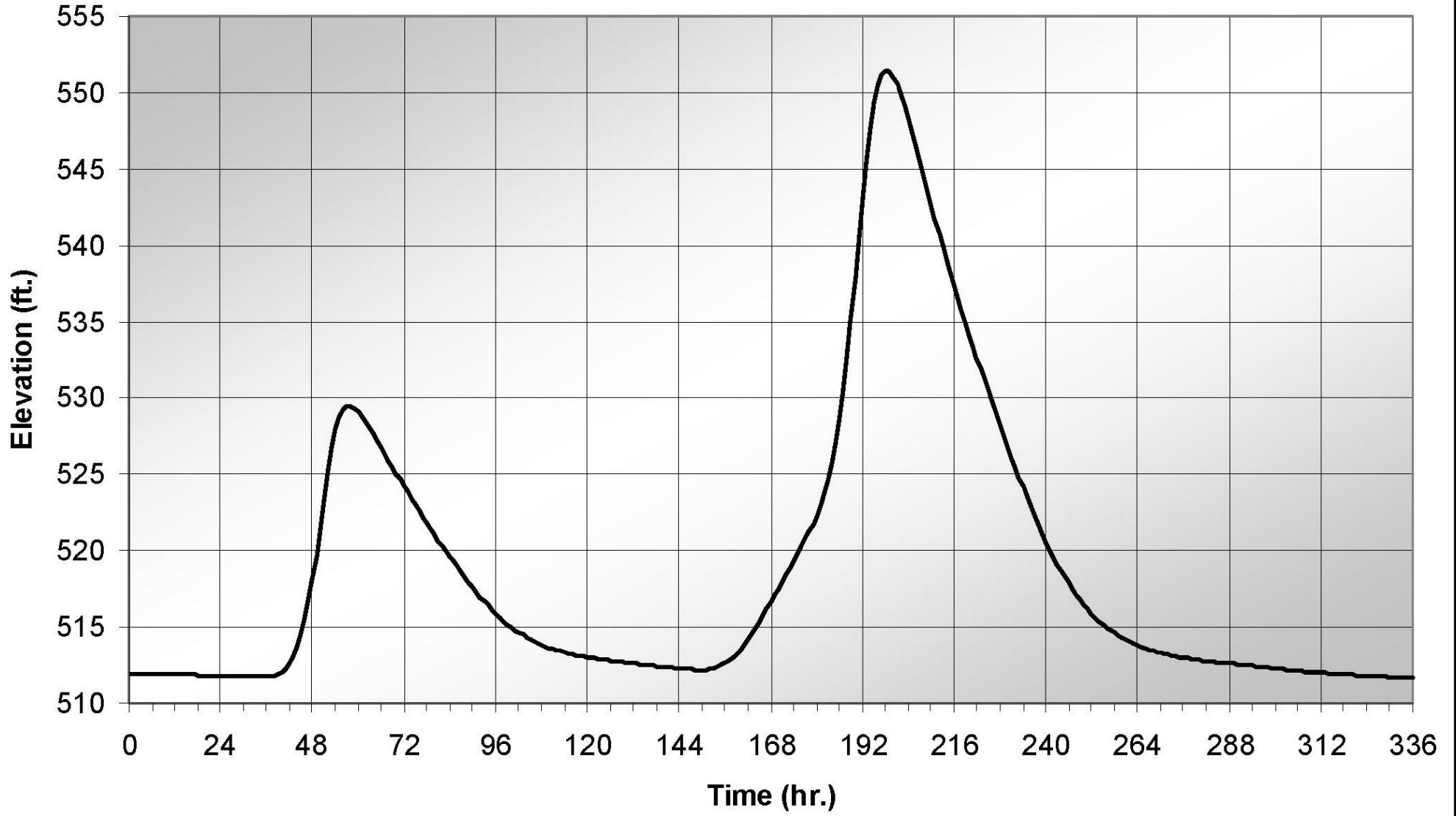
WILLIAM STATES LEE III NUCLEAR STATION UNITS 1 & 2 PMF Elevation Hydrograph, Broad River at Lee Nuclear Station FIGURE 2.4.3-229 Rev 2
