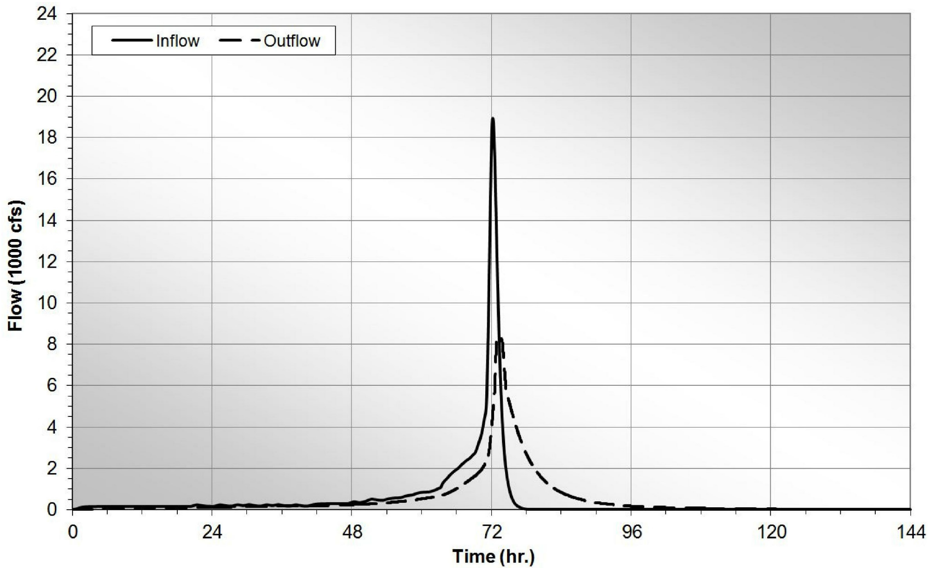
WILLIAM STATES LEE III NUCLEAR STATION UNITS 1 & 2 PMF Hydrograph Without Upper Arm Dam Failure, Make-Up Pond B FIGURE 2.4.3-227 Rev 7
