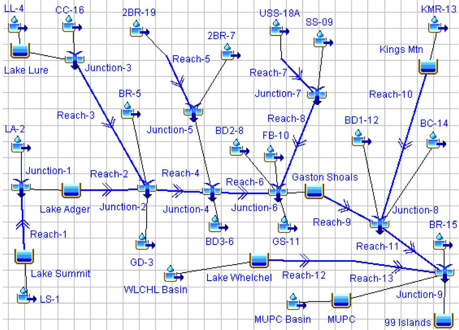
WILLIAM STATES LEE III NUCLEAR STATION UNITS 1 & 2 HEC-HMS Broad River Watershed Subbasin Schematic FIGURE 2.4.3-206 Rev 2
