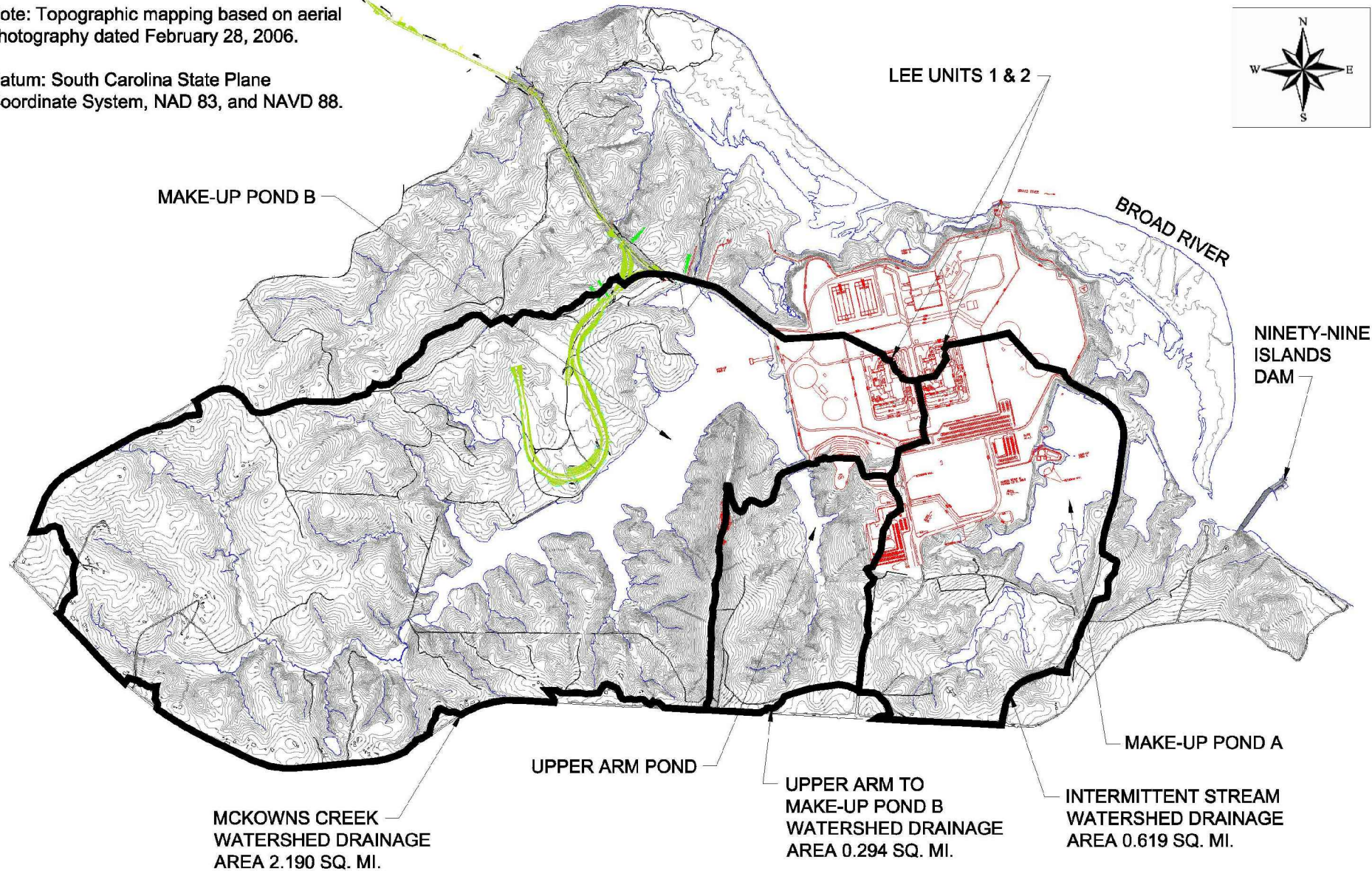
WILLIAM STATES LEE III NUCLEAR STATION UNITS 1 & 2 Make-Up Pond A and Make-Up Pond B Watersheds FIGURE 2.4.3-201 Rev 7
