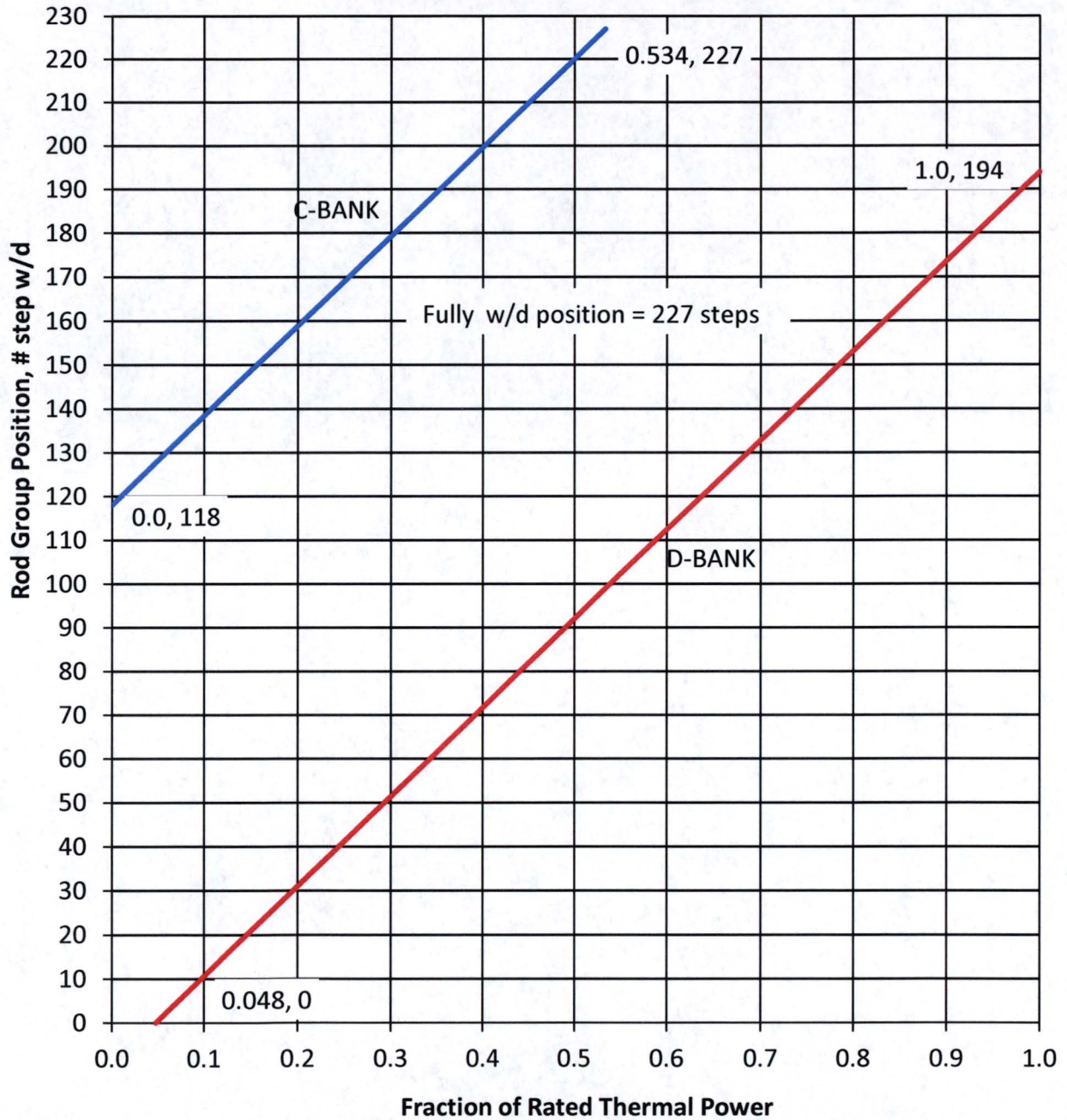
COLR Figure 3.1-1 North Anna 2 Cycle 25 Control Rod Bank Insertion Limits
